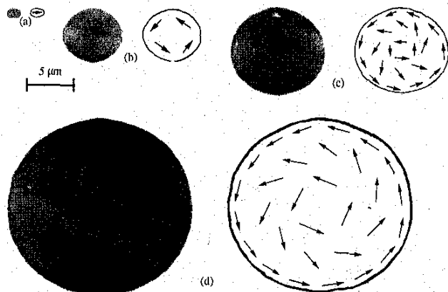
Fig. 2. MFM images and corresponding schematic magnetic domain configurations of permalloy circular disks of the size r = (a) 1 \mu\text{m} , (b) 5 \mu\text{m} , (c) 10 \mu\text{m} and (d) 20 \mu\text{m} .
