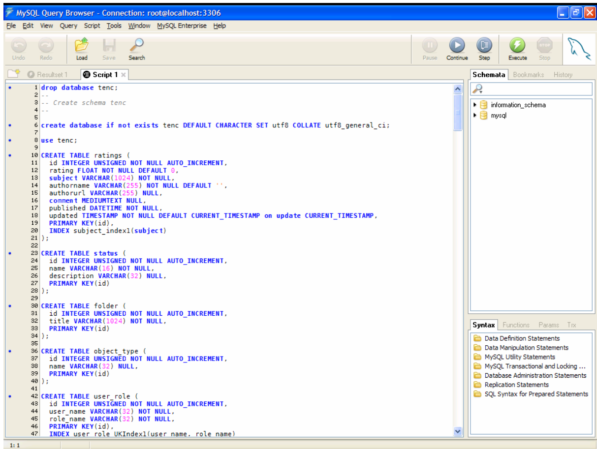
Figure 5: full_setup_db.sql file
