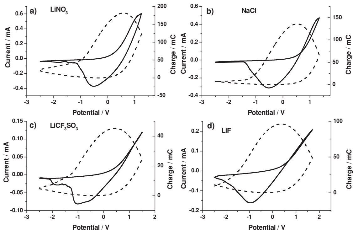
Figure 3. Voltammetric and coulometric responses of self-supported polypyrrole films in 0.1 M aqueous solutions of different salts—a) \text{LiNO}_3 , b) \text{NaCl} , c) \text{LiCF}_3\text{SO}_3 , d) \text{LiF} —at a constant sweep rate of 3 \text{ mV s}^{-1} .
