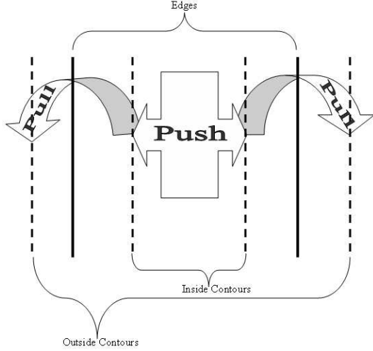
Figure 1: A Ribbon of Twin Diagram
