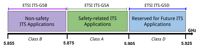
FIGURE 4: Sub-bands of the original European variant ITS-G5.
