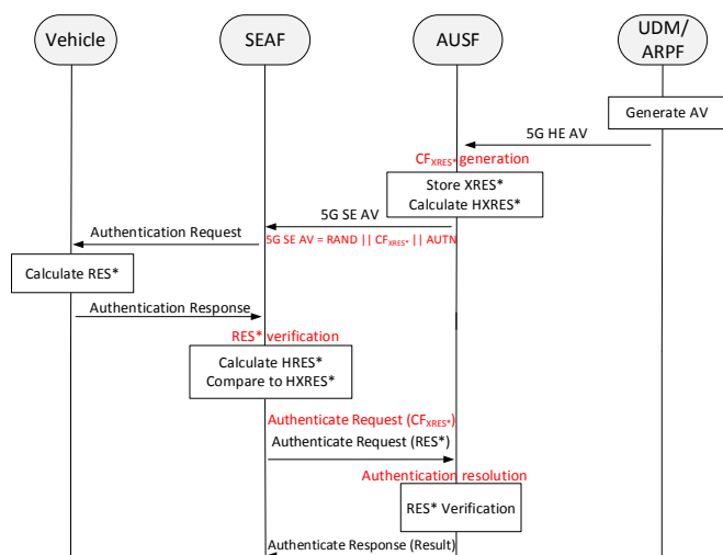
FIGURE 14: Signalling flow in standardized 5G-AKA procedure and proposed extensions (highlighted in red) in [215].
