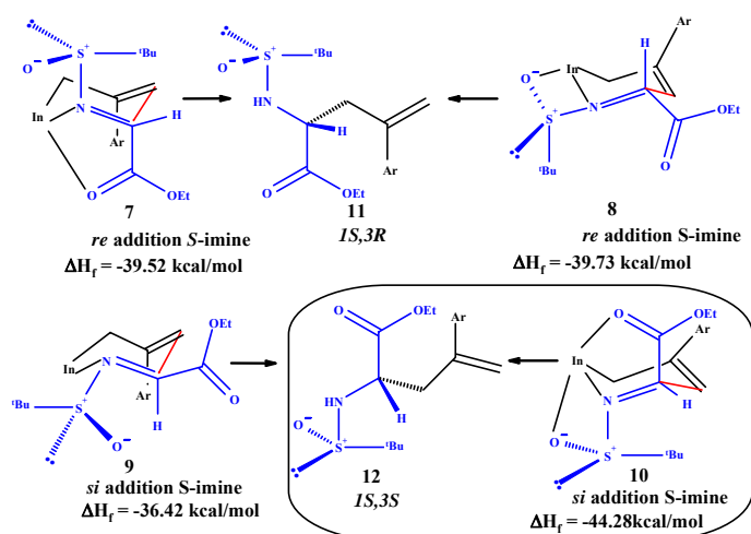
Figure 2. Stereochemical rationale for Scheme 2.
