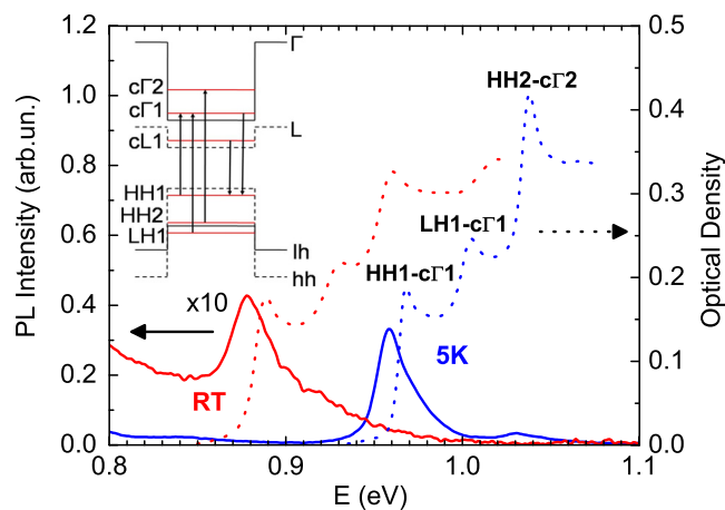
FIG. 1. (Color online) PL (full lines) and absorption (dashed lines) spectra measured at RT and at 5 K and detected by an InGaAs detector. Inset: conduction and valence band edge profiles and electron and hole confined states (energies not to scale); the transitions visible in the absorption and PL spectra are also shown.
