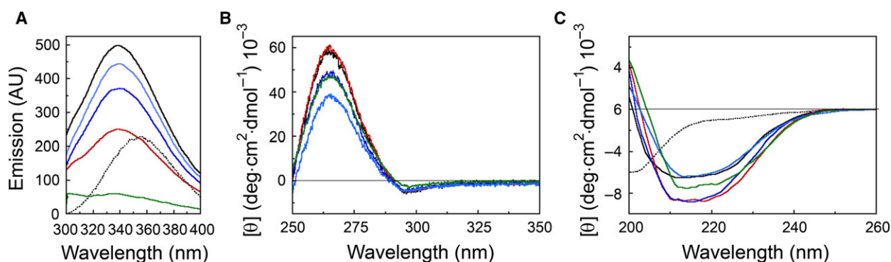
Fig. 6. Spectral properties of pLG72 variants. (A) Fluorescence spectra; (B) near-UV CD spectra; (C) far-UV CD spectra. Full-length pLG72 (black); pLG72 1–123 (blue); pLG72 1–94 (light blue); pLG72 72–153 (red); pLG72 1–64 (green); pLG72 122–153 (dotted black).
