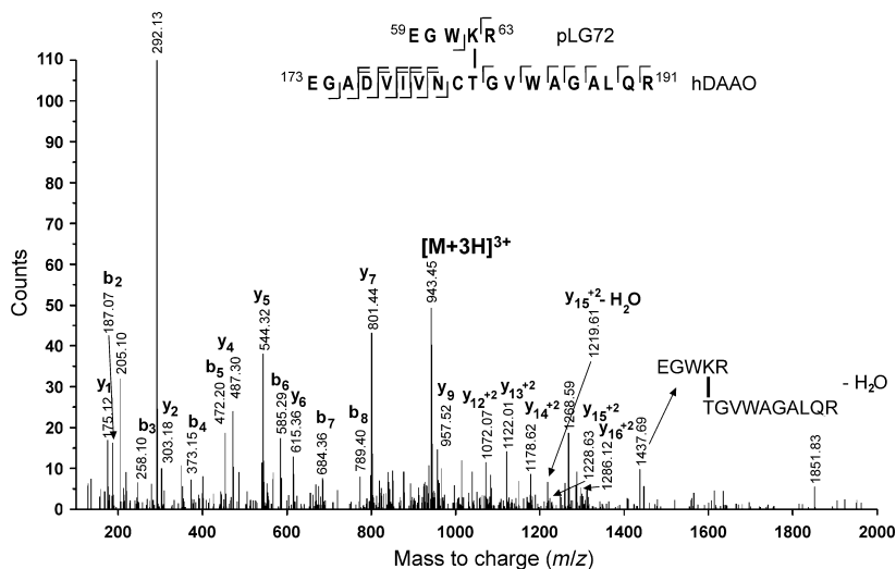
Fig. 3. MS/MS spectra of the triply charged ions at m/z 943.45 (experimental [MH]^+ m/z 2828.35, calculated [MH]^+ m/z 2828.41) interpreted as peptide 173–191 of hDAAO linked to peptide 59–63 of pLG72 (see inset). The product ions are indicated with the observed mass.
