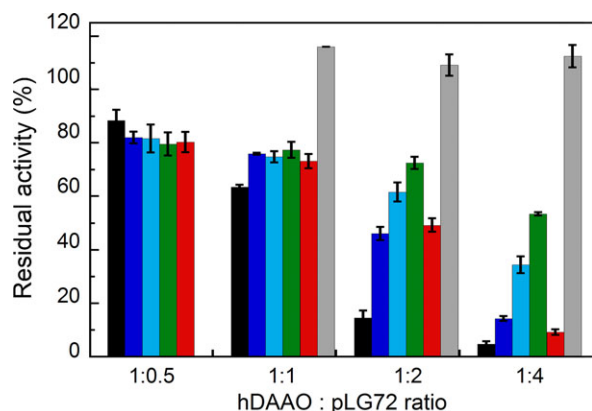
Fig. 8. Effect of increasing amounts of pLG72 on the activity of hDAAO. The residual activity was assayed 30 min after incubation of 13 \mu\text{M} hDAAO and pLG72 (at the indicated molar ratios), at 25 °C. The activity of hDAAO alone is referred as 100%. Full-length pLG72 (black); pLG72 1-123 (blue); pLG72 1-94 (light blue); pLG72 1-64 (green); pLG72 72-153 (red); pLG72 122-153 (gray). n.d. = not determined. Bars represent mean \pm SD, n = 4 .
