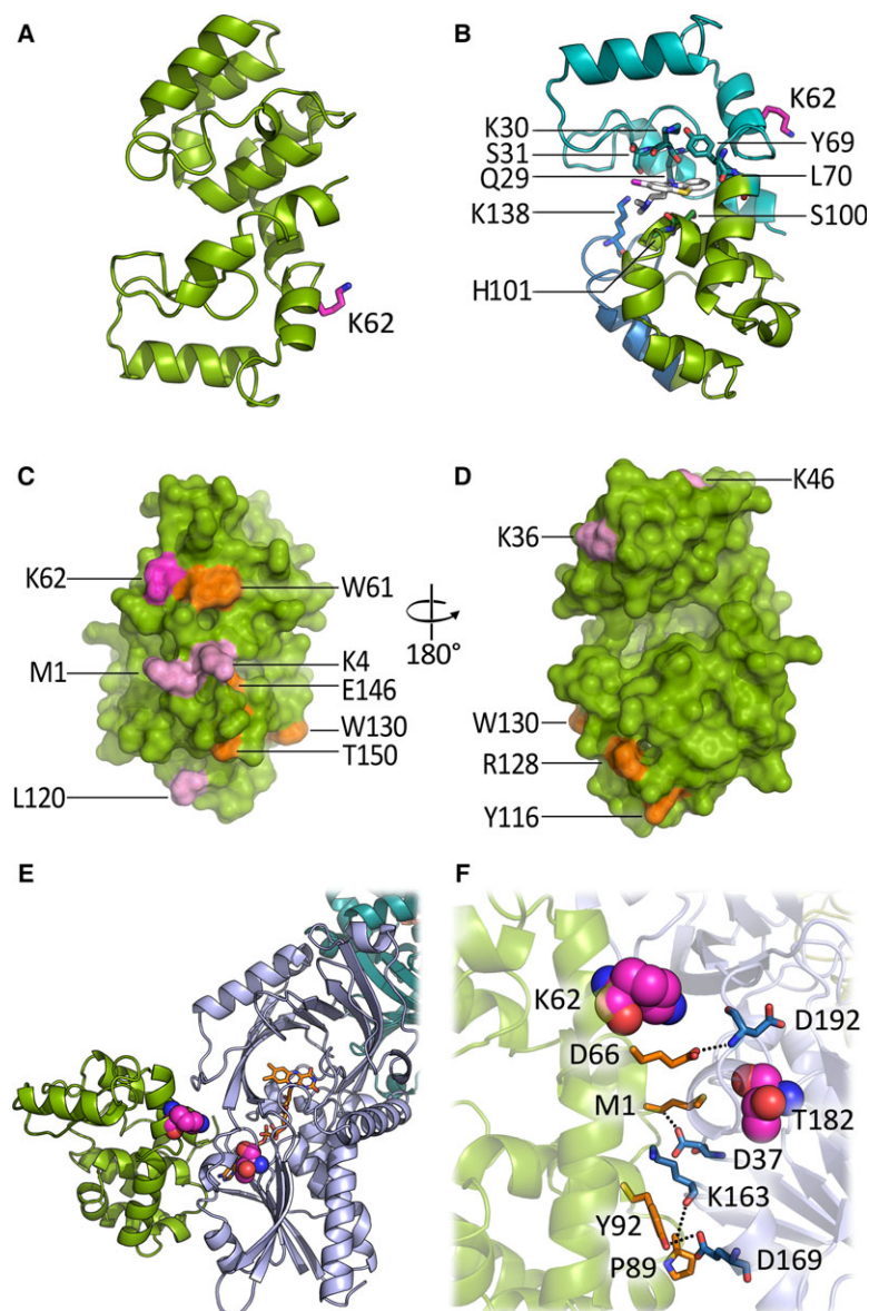
Fig. 4. Homology model of pLG72 and proposed mode of interaction with CPZ and hDAAO. (A) Model of pLG72-VA, produced by I-TASSER server using the structure of T4 lysozyme (pdb code 2171) as template; residue K62, identified by cross-linking experiments with hDAAO, is represented in purple. (B) Mode of CPZ binding to pLG72-VA obtained by automated molecular docking simulations using AUTODOCK VINA [50]; the ligand is shown in van der Waals and sticks representation (white atoms), orientation of pLG72-VA is reversed in comparison with panel A. The dark blue depicts the region deleted in pLG72 1–123 , and light blue depicts the region deleted in pLG72 72–153 . Residues forming noncovalent interactions with CPZ are shown as sticks. (C) Surface representation of pLG72-VA model: proteolytic sites are shown in orange, dead-end modified residues by BS 3 are shown in pink and cross-linked K62 residue is shown in purple. M1 and K4 form an intramolecular cross-link (see Tables 1 and 2 for details). (D) Model of hDAAO–pLG72 complex as predicted by ZDOCK server; pLG72-VA is in green, hDAAO monomers in violet and cyan. (E) Details of the H-bonds formed at the contact interface. Residues identified by cross-linking experiments are shown in van der Waals radius representation, and residues forming H-bonds at the interface are shown as sticks; dotted lines represent hydrogen bonds.
