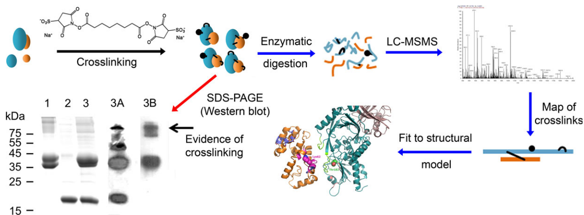
Fig. 2. Scheme of the strategy employed for the identification of the regions involved in hDAAO-pLG72 complex formation by means of cross-linking based on SB 3 . Red arrow: gel-based approach showing the electrophoretic analysis of 12.5 \mu M hDAAO (lane 1), 62.5 \mu M pLG72 (lane 2), and the corresponding hDAAO-pLG72 complex (at 1 : 5 subunit molar ratio, lane 3) incubated for 15 min and then cross-linked by adding 625 \mu M SB 3 . Lane 3 was also analyzed by western blot using anti-hDAAO (3A) and anti-pLG72 antibodies (3B): besides some protein bands related to intramolecular cross-links occurring within both hDAAO and pLG72, immunodetection analyses revealed that the band at ~ 75 kDa (arrow) was positive to both antibodies. Blue arrows: in solution, gel-free procedure.
