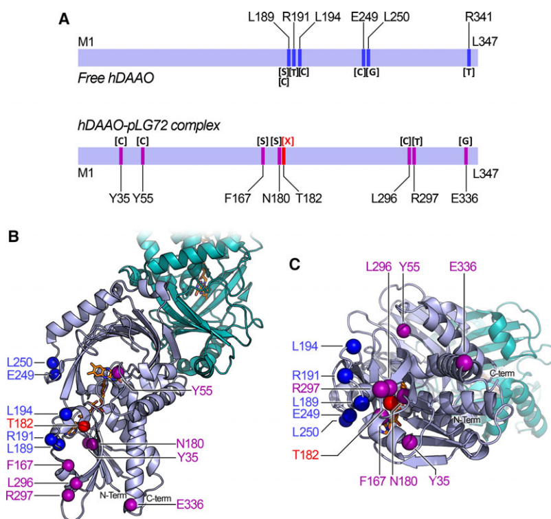
Fig. 1. Proteolysis of hDAAO. (A) Schematic representation of preferential proteolytic sites in hDAAO alone and in the presence of pLG72 (indicated by blue and purple bars, respectively). C = chymotrypsin; S = subtilisin; T = trypsin; G = endoprotease Glu-C; X = SB 3 cross-link (red bar). (B, C) Representation of the sites of proteolysis (spheres) within the three-dimensional structure of hDAAO homodimer (pdb code 2du8); colors as in panel A.
