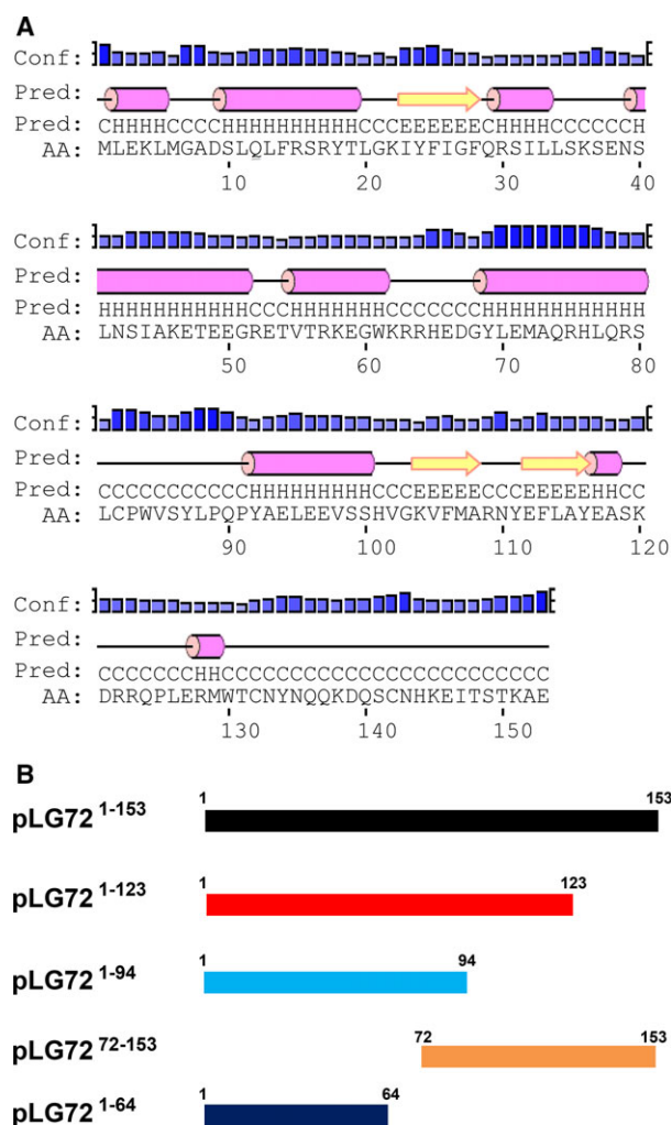
Fig. 5. Deletion variants of pLG72. (A) Pspred analysis of disordered regions in pLG72. Conf = confidence of prediction; C = coil; E = strand; H = helix. (B) Schematic representation of the pLG72 variants produced in this work.
