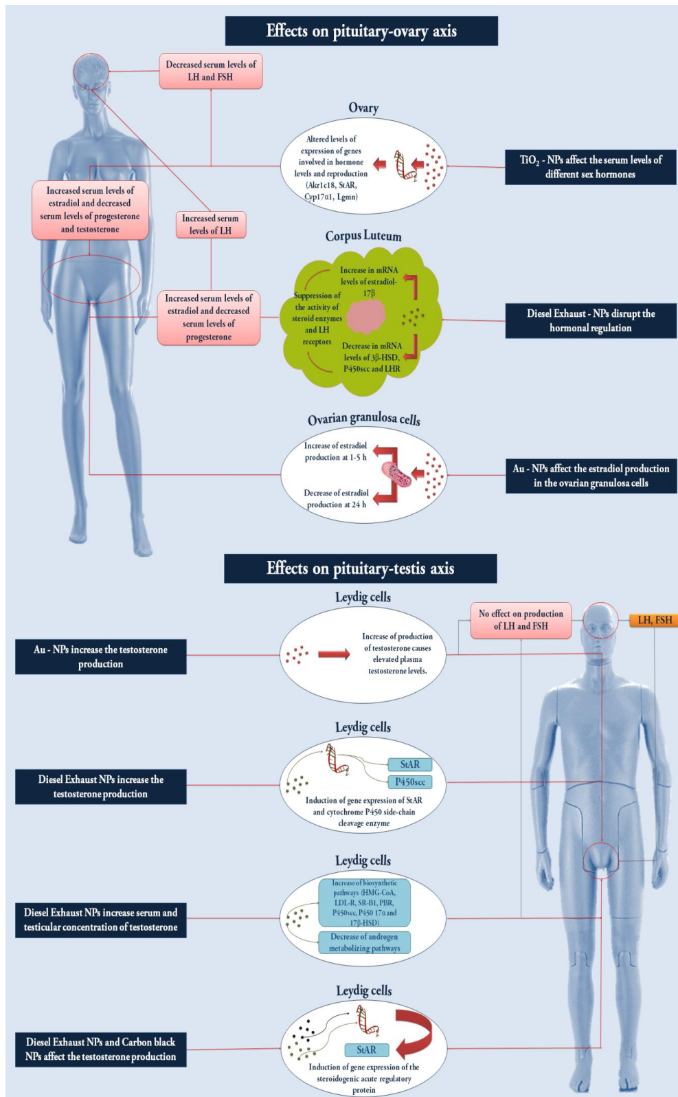
Figure 2. Effects on pituitary-ovary and pituitary-testis axes caused by exposure to different types of NPs.
