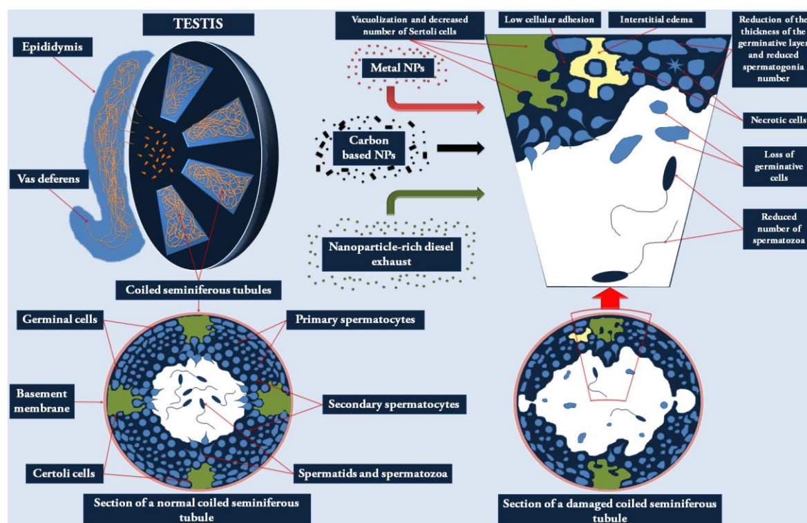
Figure 1. Alterations and impairment of testicular structure induced by exposure to different types of NPs. Metal-based NPs, carbon-based NPs and nanoparticle-rich diesel exhaust (NRDE-NPs) were reported to induce changes in testicular histology of laboratory animals. Metal-based NPs (TiO 2 -NPs) induced the disruption of seminiferous tubules and decreased the number of Sertoli cells; Carbon-based NPs (carbon black-NPs, multi-walled carbon nanotubes) caused vacuolization of seminiferous tubules, seminiferous tubule damage and low cellular adhesion of seminiferous epithelia, partial disappearance or vacuolization of Sertoli cells, reduced thickness of the germinative layer, lower spermatogonia number, vasodilatation and hyperemia; NRDE-NPs induced degenerative and necrotic changes, interstitial edema, desquamation of the seminiferous epithelium, loss of germ cells and spermatozoa.
