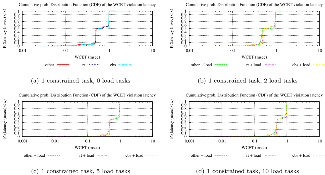
Figure 6: Cumulative Distribution Function (CDF) of all the notifications of a WCET violation of the all the various experiments.
