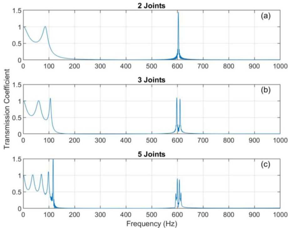
Fig. 8. Transfer functions for identical rock masses ( s = 2 m, C_p = 2365 m/s, C_s = 1922 m/s, k_n = 1 GPa/m, \rho = 2600 kg/m 3 ) with different numbers of joints: (a) 2 joints, (b) 3 joints, and (c) 5 joints.
