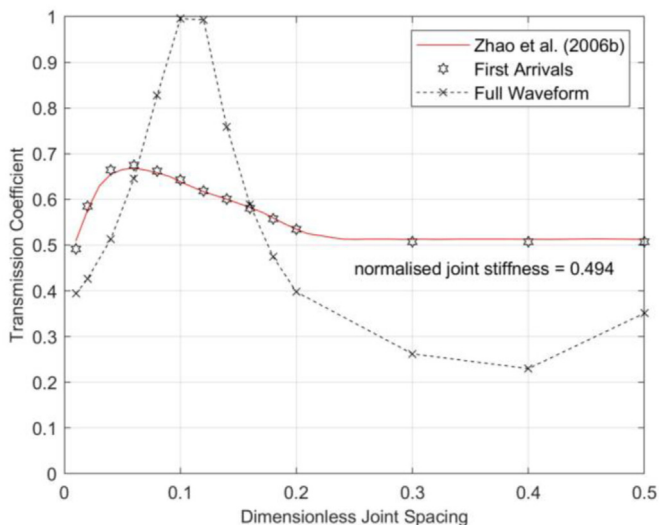
Fig. 12. Transmission coefficients for jointed rocks with J_n of 2, plotted against dimensionless joint spacing ( \xi ) with results from Zhao et al. (2006b) and from the current study generated using the first arrival and the full waveform.
