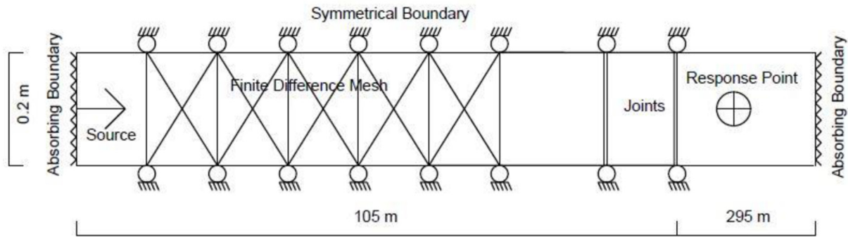
Fig. 2. UDEC model showing finite difference mesh. Mesh fills entire model. Not to scale.
