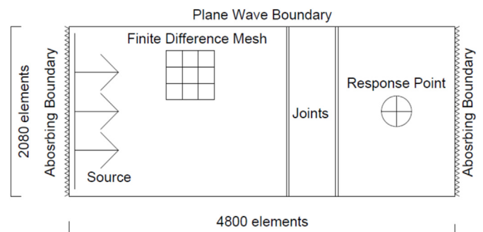
Fig. 3. WAVE2D model showing finite difference mesh. Mesh fills entire model. Not to scale.
