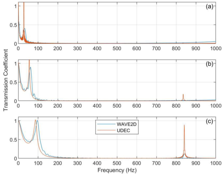
Fig. 5. High density ( 26,000 \text{ kg/m}^3 ) transfer functions from WAVE2D and UDEC for a material with C_p of 3328 m/s and C_s of 1922 m/s: (a) k_n = 1 GPa/m, (b) k_n = 4 GPa/m, and (c) k_n = 10 GPa/m.
