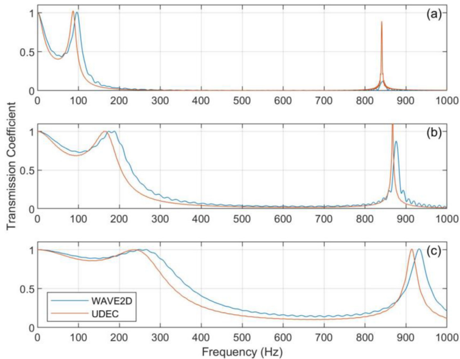
Fig. 6. Medium density ( 2600 \text{ kg/m}^3 ) transfer functions from WAVE2D and UDEC for a material with C_p of 3328 m/s and C_s of 1922 m/s: (a) k_n = 1 GPa/m, (b) k_n = 4 GPa/m, and (c) k_n = 10 GPa/m.
