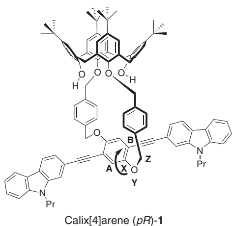
Fig. 5 Assignment of configuration to ICC 1 .
