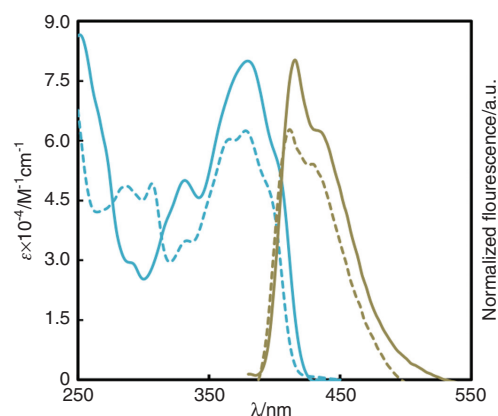
Fig. 3 Absorption and fluorescence spectra of calix[4]arenes 1 (solid line) and 2 (dashed line) in \text{CHCl}_3 (298 K; \lambda_{\text{exc}} = 380 nm).
