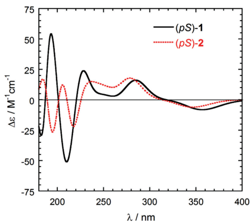
Fig. 9 CD spectra calculated at CAM-B3LYP/SV//B3LYP/6-311G* level in vacuo for (pS) - 1 and (pS) - 2 . Each spectrum is the arithmetic average of four representative structures (see text); Gaussian band-shape with 0.25 eV exponential half-width.
