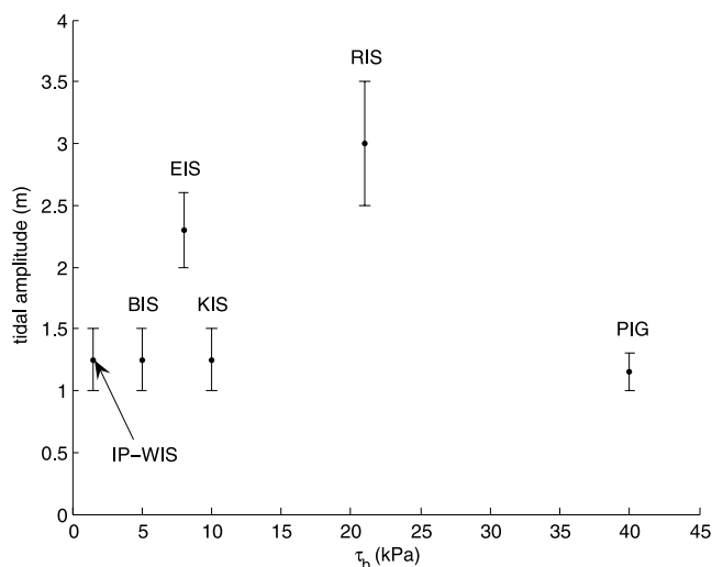
Figure 4. Basal shear stress ( \tau_b ) and tidal amplitude at spring tide for a number of West Antarctica ice streams. Abbreviations used are PIG for Pine Island Glacier, RIS for Rutford Ice Stream, KIS for Kamb Ice Stream, EIS for Evans Ice Stream, BIS for Bindschadler Ice Stream, and IP-WIS for the ice plain of Whillans Ice Stream. Basal shear stresses given are approximates, and true basal shear stresses vary significantly within each ice stream [Joughin et al. , 2004]. Tidal ranges were calculated using the CATS02.01 tidal model [Robertson et al. , 1998] (see http://www.esr.org/ptm_index.html ). Basal shear stress estimates are derived from Raymond [2000] and Joughin et al. [2004].
