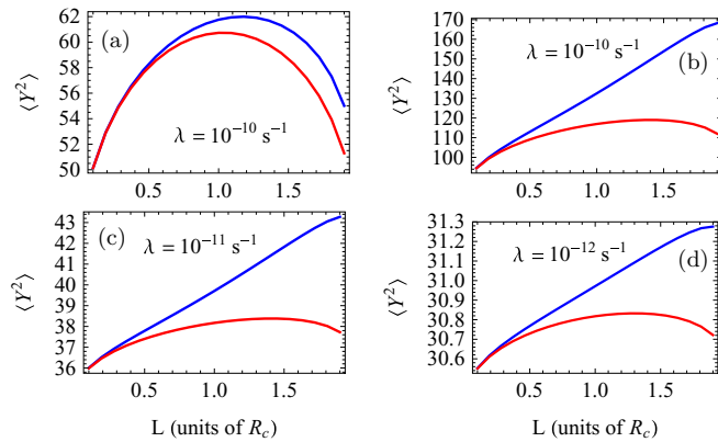
FIG. 3. Steady-state variance of the optical phase quadrature \langle Y^2 \rangle vs the cavity length L with (a) \omega = \Delta = 0.02\kappa , G = 0.15\kappa , P_a = 10^{-10} Torr, (b) \omega = \Delta = 0.008\kappa , G = 0.08\kappa , P_a = 10^{-10} Torr, (c) \omega = \Delta = 0.008\kappa , G = 0.025\kappa , P_a = 10^{-11} Torr, and (d) \omega = \Delta = 0.008\kappa , G = 0.009\kappa , P_a = 10^{-12} Torr. The values of \lambda are reported in each plot. All the curves are evaluated for T = 100 mK and R_c = 2 cm, and the other parameters are as in Fig. 2. Blue (red) lines represent the case with (without) the CSL effect.
