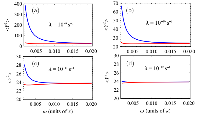
FIG. 2. Steady-state variance of the optical phase quadrature \langle Y^2 \rangle vs the trapping frequency \omega for (a) \lambda = 10^{-9} s ^{-1} , T = 200 mK, P_a = 10^{-10} Torr, (b) \lambda = 10^{-10} s ^{-1} , T = 100 mK, P_a = 3 \times 10^{-11} Torr, (c) \lambda = 10^{-11} s ^{-1} , T = 60 mK, P_a = 10^{-11} Torr, and (d) \lambda = 10^{-12} s ^{-1} , T = 10 mK, P_a = 10^{-12} Torr. Blue (red) lines represent the case with (without) the CSL effect. In all plots we take G = 0.001\kappa . The other parameters are as in Fig. 1(b).
