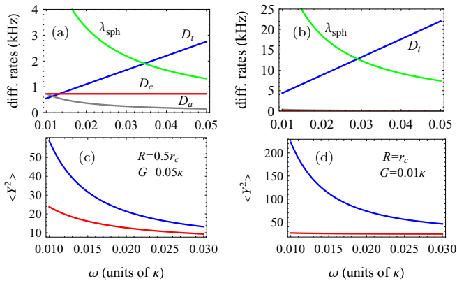
FIG. 1. (a), (b) Diffusion rates for the scattering of trapping light D_t (blue), cavity light D_c (red), air molecules D_a (gray), and the collapse rate \lambda_{\text{sph}} (green) vs the mechanical frequency \omega with (a) R = 0.5r_c and G = 0.05\kappa , (b) R = r_c and G = 0.01\kappa . Note that the curves of D_c and D_a in (b) are very close to the \omega axis and no longer visible. (c), (d) Steady-state variance of the optical phase quadrature \langle Y^2 \rangle vs the trapping frequency \omega . Blue (red) lines refer to the case with (without) the CSL effect. The parameters for (c) [(d)] correspond to those for (a) [(b)]. The other parameters are L = R_c = 1 cm, \mathcal{F} = 10^5 (corresponding to \kappa = 0.47 MHz), \Delta = 0.01\kappa , \lambda_c = 1064 nm, \mathcal{N} = 0.6 , T = 1 K, P_a = 10^{-10} Torr, \lambda = 10^{-8} s ^{-1} , r_c = 100 nm, and we consider a diamond nanosphere with \rho_0 = 3.5 g/cm ^3 and \epsilon = 5.76 .
