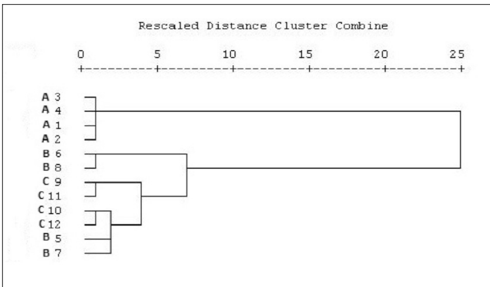
Fig. 1. Dendrogram of Tuber spp. hexane extract with fatty acids contents. A1-A4: Tuber aestivum , B5-B8: T. uncinatum , C9-C12: T. melanosporum .
