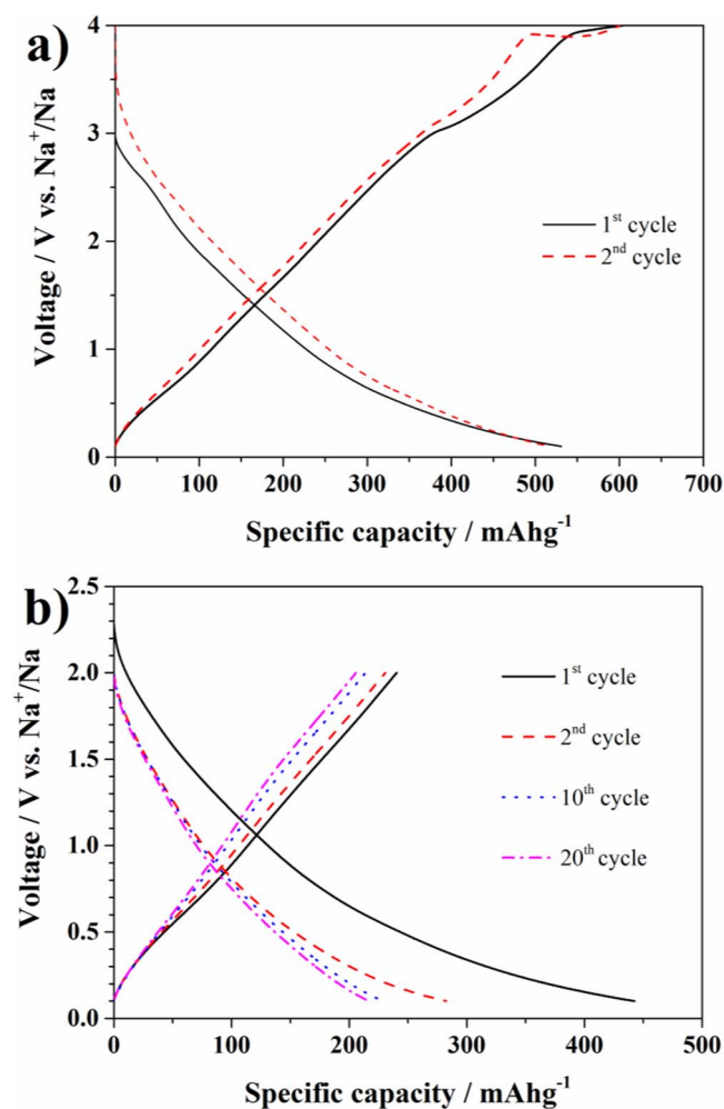
Figure 2. (a) Voltage profile of V_2O_5 aregel electrode upon the initial two cycles at current density of 14.7 \text{ mA g}^{-1} ( 0.1 \text{ C} ) in the voltage range 0.1 V–4 V vs Na/Na^+ . (b) Selected voltage profiles of the V_2O_5 electrode cycled at C/10 in the voltage range 0.1 V–2 V vs Na/Na^+
