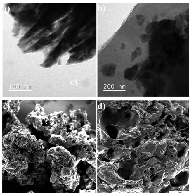
Figure 4. C-coated Na_3V_2(PO_4)_3 powder. (a-b) TEM and (c-d) SEM images, at different magnification level.
