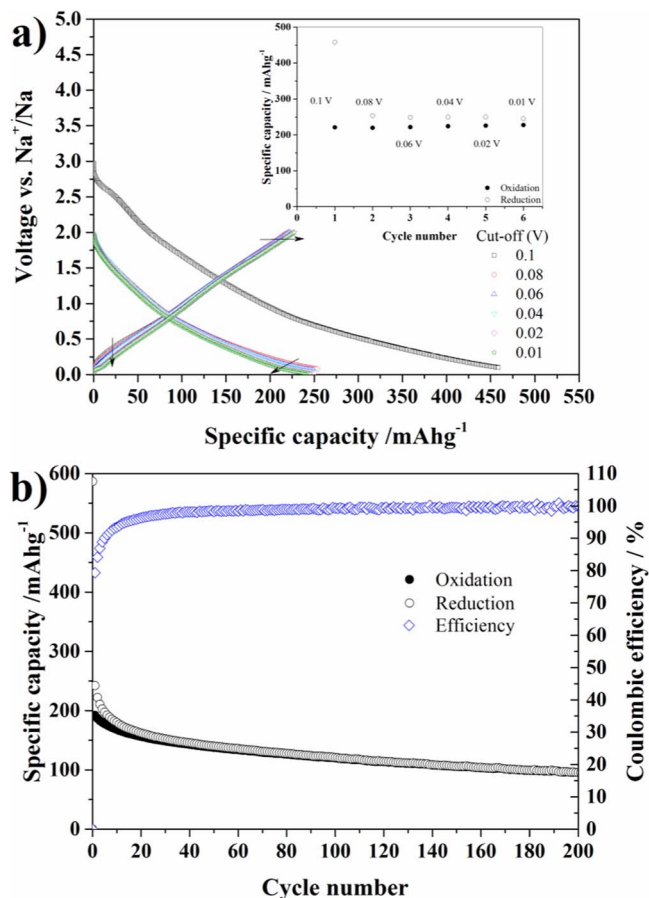
Figure 3. (a) Voltage profile of a V_2O_5 aerogel electrode obtained at 74 mAg^{-1} ( C/2 ) using progressively lower (the upper cut-off is fixed at 2 V vs Na/Na^+ ). The inset shows the capacity delivered for each cycle at specific cutoff. (b) Long-term performance of V_2O_5 aerogel electrode upon continuous cycling at 100 mA g^{-1} in the voltage range 0.01 V–1.5 V vs Na/Na^+ .
