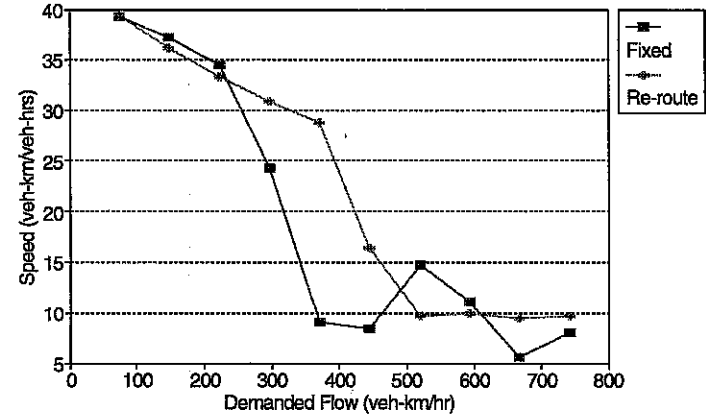
Ring-Radial 9 Zone ODB : Slice 2+3 Speed vs Demanded Flow Zone 2 Outbound
