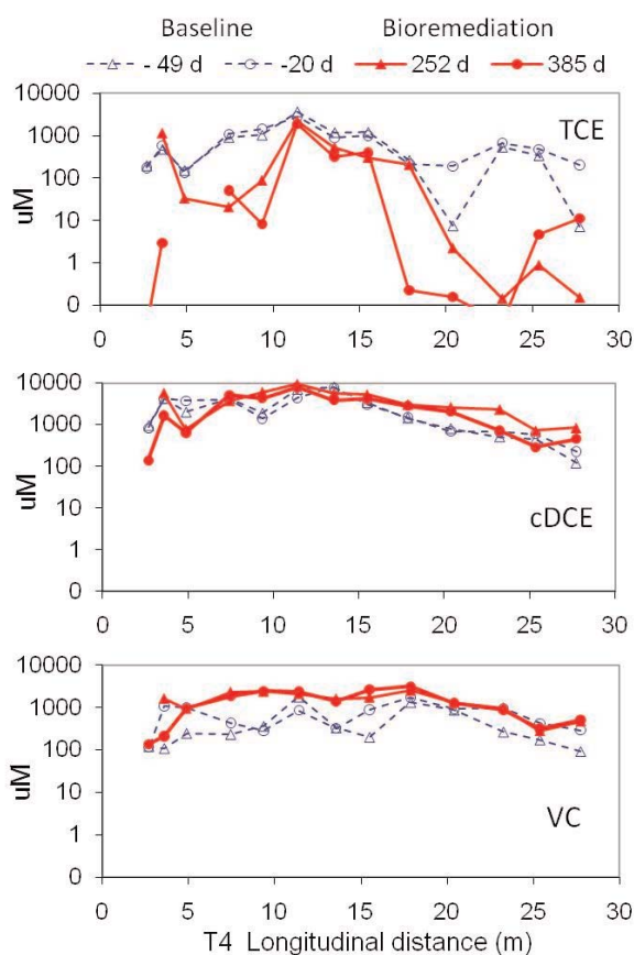
Figure 4. Example longitudinal concentration profiles based on averaged T4 MLS concentration data.
