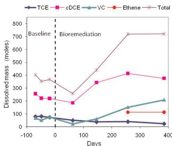
Figure 5. Estimated cell dissolved-phase mass with time estimated from the T4 transect data.
