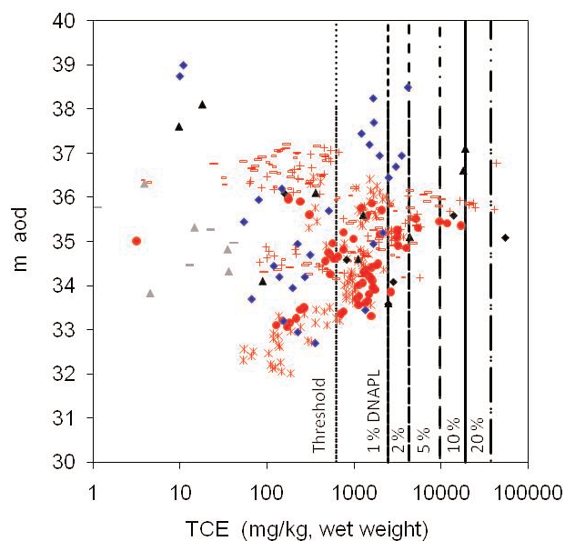
Figure 2. Pre-baseline TCE soil-concentration depth profiles for the T1 transect (red symbols) and T4 transect (other colour symbols, and red-filled circles for the T1 - T4 intersection profile).
