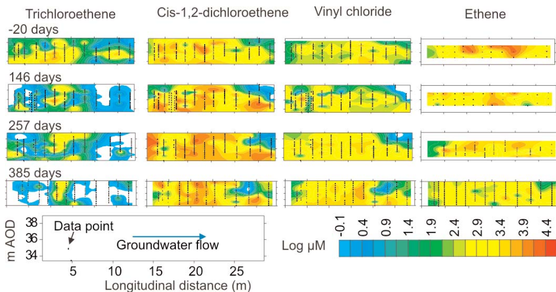
Figure 3. Example dissolved plume MLS snapshot data collected from T4 during the baseline and bioremediation phase.
