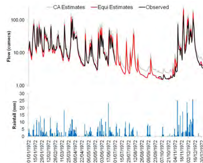
Figure 6 Top: Observed 1972 flows for the South Tyne at Haydon Bridge (23004) and estimated flows under equipercentile and CA techniques, based upon donor of South Tyne at Featherstone (23006). Bottom: Rainfall from the Met Office rain gauge 14284.
