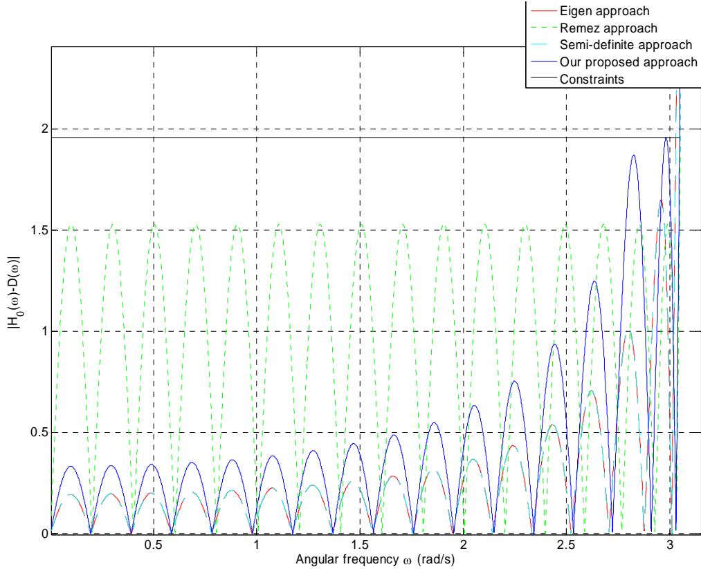
Figure 2. Weighted error function of the full band fifth order differentiators.
