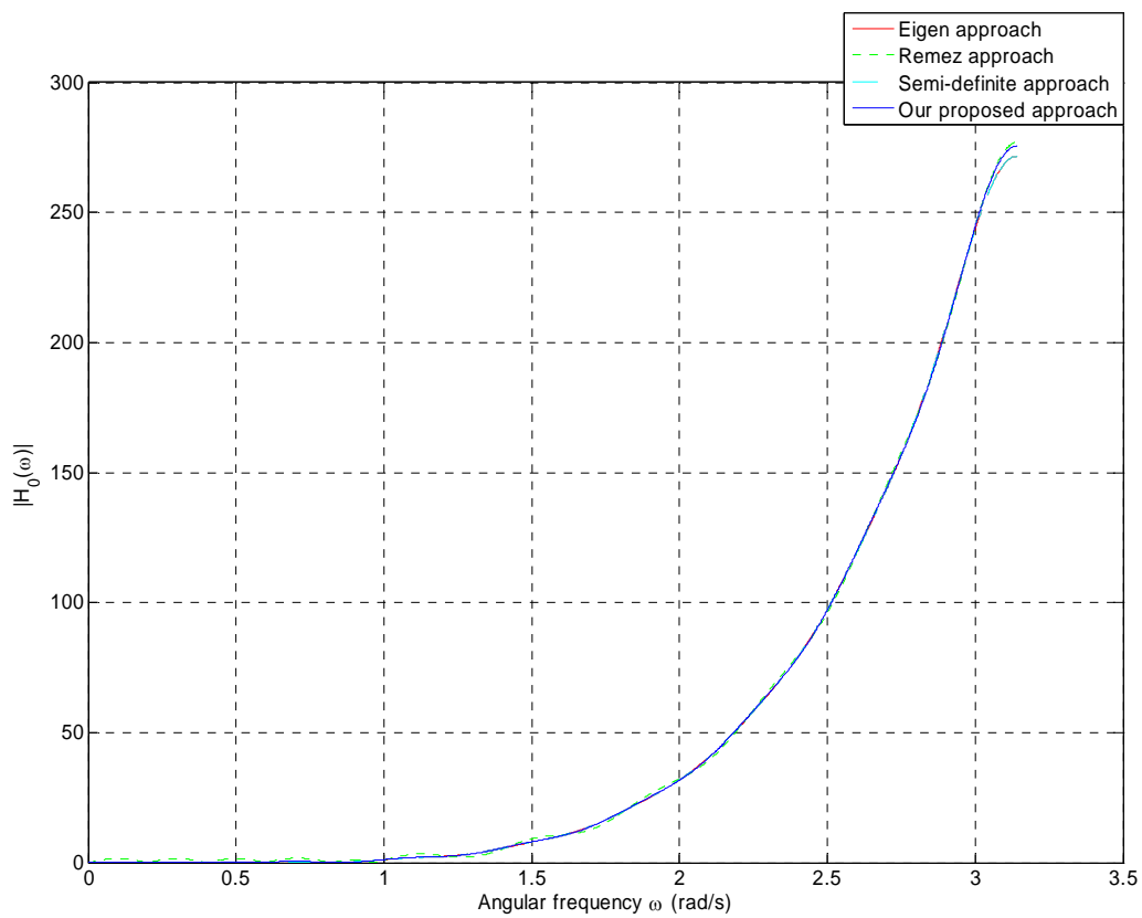
Figure 1. Magnitude response of the full band fifth order differentiators.
