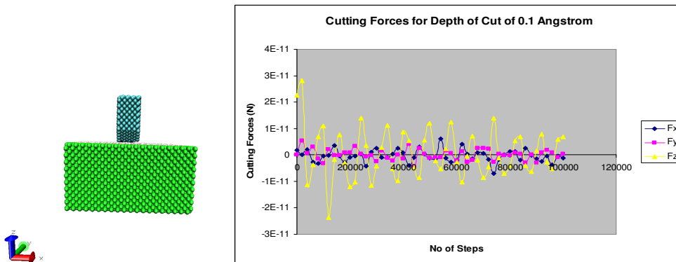
Figure 1: Depth of Cut and Cutting Forces for Depth of Cut - 0.1 Å
