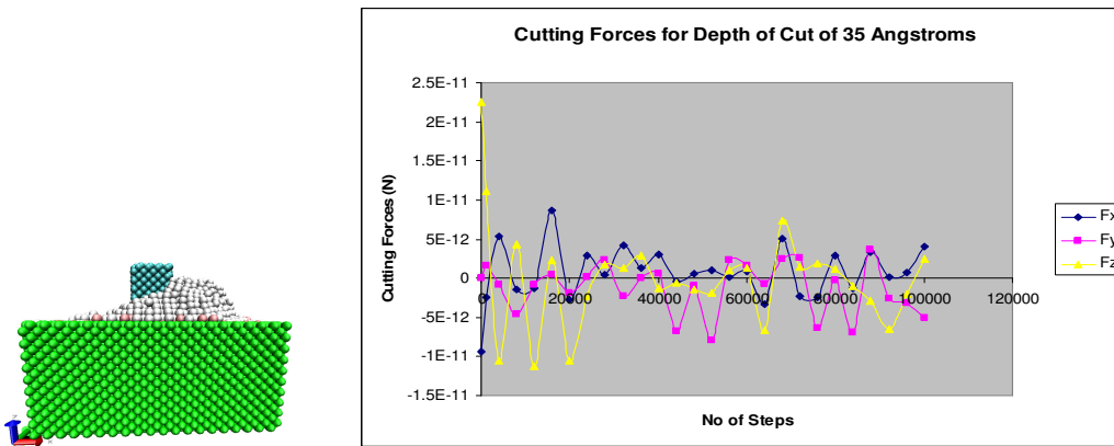
Figure 4: Depth of Cut and Cutting Forces for Depth of Cut – 35.0 Å
