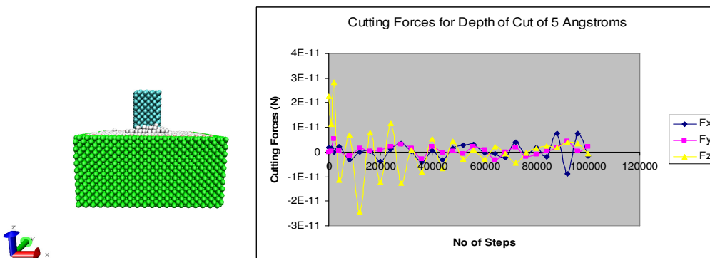
Figure 2: Depth of Cut and Cutting Forces for Depth of Cut – 5.0 Å
