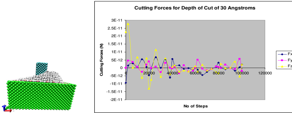
Figure 3: Depth of Cut and Cutting Forces for Depth of Cut – 30.0 Å
