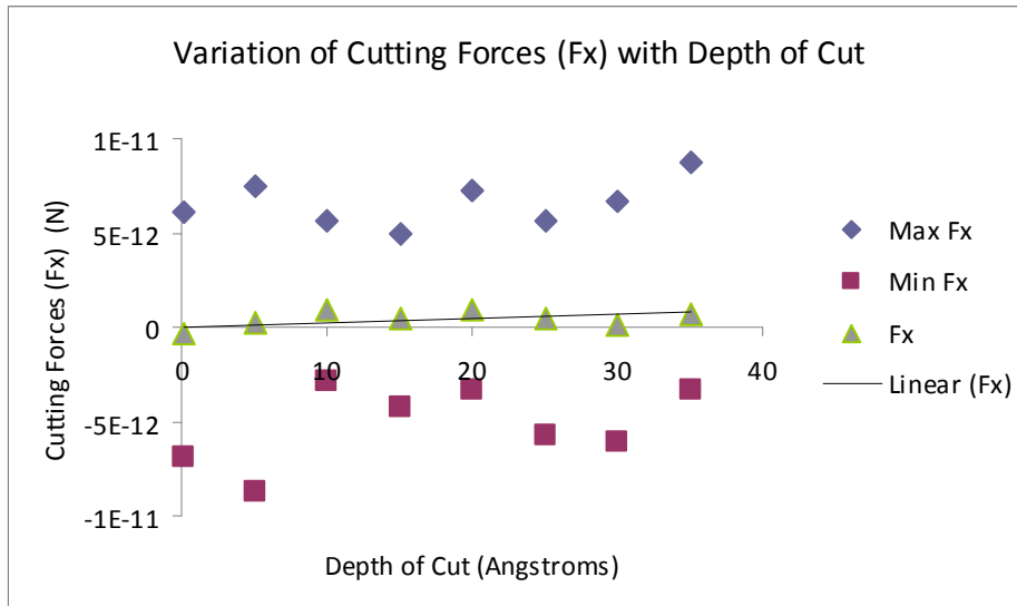
Figure 5: The Variation of Cutting Forces with Depth of Cut
