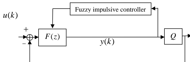
Figure 2. The block diagram of the interpolative SDM under the fuzzy impulsive control strategy.
