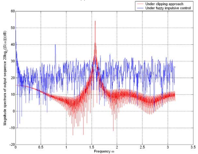
Figure 6: Magnitude response of the output sequence when \bar{u}=0.75 and initial condition \tilde{\mathbf{x}}(0)=[0, 0, 0, 0, 0]^T for both the clipping and fuzzy impulsive control strategies are applied with the state variables bounded by 40.
