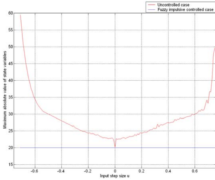
Figure 3: Plot of the maximum absolute value of the state variables (realized in direct form) against the input step size when \tilde{\mathbf{x}}(0)=[0, 0, 0, 0, 0]^T .
