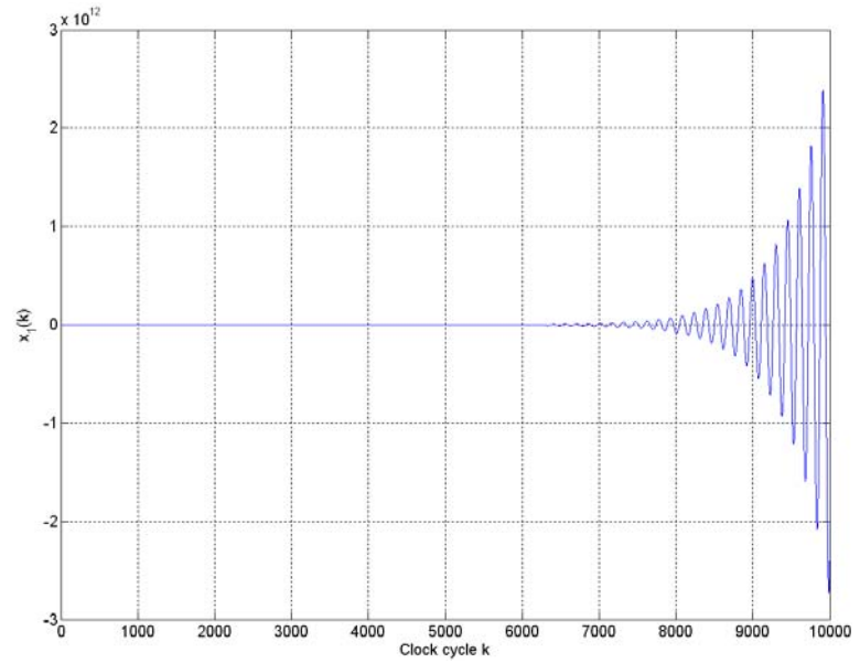
Figure 5: The response of x_1(k) with input step size \bar{u}=0.75 and initial condition \mathbf{x}(0)=[0, -5, 28.5, 32.25, 35.9793, 39.5612]^T when the time delay feedback control strategy with K_c=2 \times 10^{-5} is applied.
