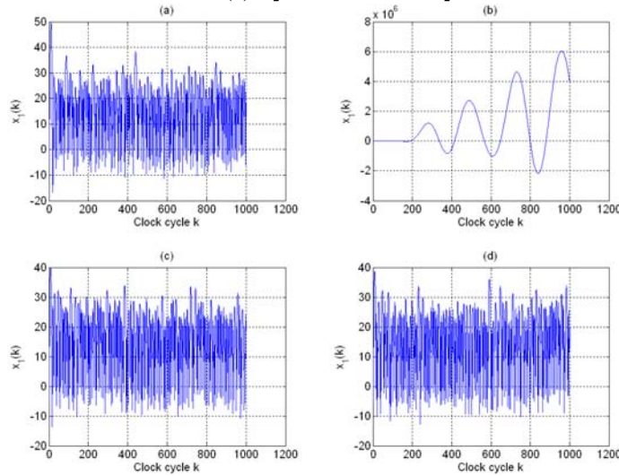
Figure 4: The response of x_1(k) when \bar{u}=0.75 and (a) initial condition \tilde{\mathbf{x}}(0)=[0, 0, 0, 0, 0]^T when no control strategy is applied. (b) initial condition \tilde{\mathbf{x}}(0)=[0.001, 0, 0, 0, 0]^T when no control strategy is applied. (c) initial condition \tilde{\mathbf{x}}(0)=[0, 0, 0, 0, 0]^T when the fuzzy impulsive control strategy with V_{cc}=40 is applied. (d) initial condition \tilde{\mathbf{x}}(0)=[0.001, 0, 0, 0, 0]^T when the fuzzy impulsive control strategy with V_{cc}=40 is applied.
