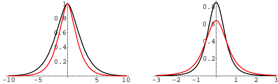
Figure 2: Ornstein–Uhlenbeck process driven by a Laplace noise: characteristic functions (left) and density functions (right) of the stationary distribution (black lines), compared with the characteristic functions and density functions of the Laplace law \mathcal{L}(a) generating the driving noise (red lines). Here a = 1/\sqrt{2} and b = 1 so that both the variances (that of the stationary distribution, and that of \mathcal{L}(a) ) are equal to 1.
