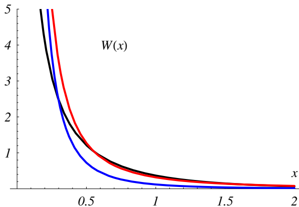
Figure 1: Densities W(x) of the Lévy measures for the selfdecomposable laws \mathcal{L}(a) (black), \mathcal{C}(a) (red) and \mathcal{S}(a) (blue). To make the plots comparable we have chosen a = 1 for all the three densities, and to make the differences more visible we have plotted only the positive x -axis since the curves are exactly symmetric on the negative axis.
