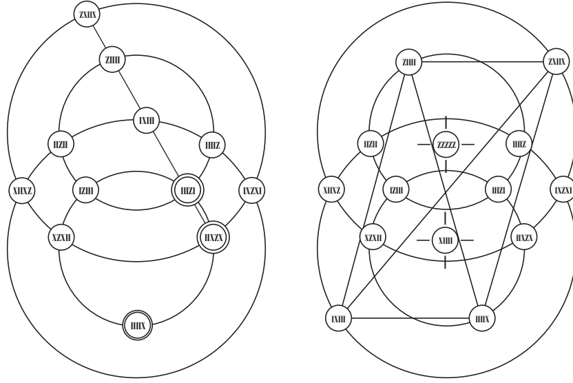
Figure 2. Left: – An illustration of the relations between the five sets of five-qubit observables of (2). Two big concentric circles at the top represent sets A and B , those at the bottom sets A' and B' ; set C is represented by the line-segment. The three “exceptional/distinguished” observables are indicated by small double-circles. Right: – The same for the five sets of (1); note that this latter configuration is more symmetric than the former one. In this section, we use a full-fledged labeling of the observables and a shorthand notation for the tensor product, e.g. XZXII \equiv X \otimes Z \otimes X \otimes I \otimes I .
