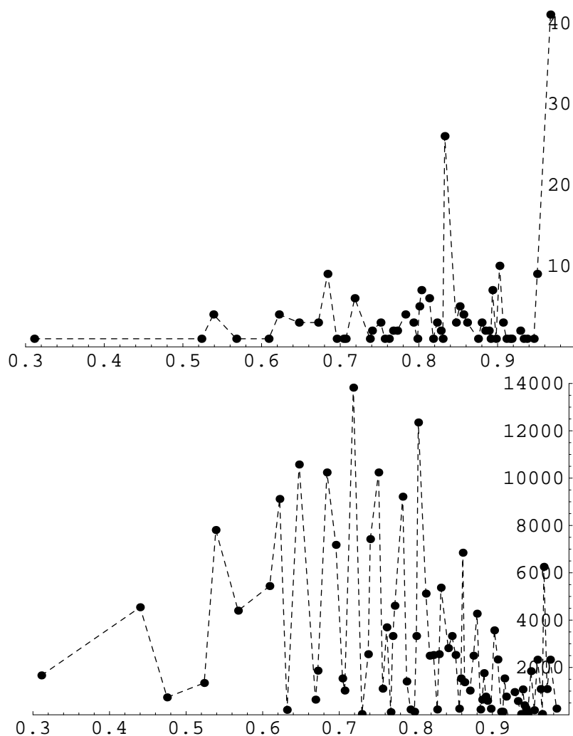
Figure 1. Top: – A histogram of distances between the maximal bases for the 160–21 proof of the BKS theorem. There are two main peaks located at d_1 = (29/31)^{1/2} \sim 0.9672 and d_2 = (43/62)^{1/2} \sim 0.8328 , but the distances are spread over 54 distinct values exhibiting a noise-like distribution; this is quite remarkable given the fact that the graph described in Sec. 2.1 possesses a rather high degree of symmetry, \mathbb{Z}_2^5 \times \mathbb{Z}_6 . Bottom: – A histogram of distances between the maximal bases for the 160–661 proof. Here the distances acquire as many as 77 distinct values, whose distribution looks again like a noise. Comparing with the top figure, one observes that a bunch of peaks in the middle range of distances is redundant for the present BKS proof because the characteristic peaks at d_1 and d_2 are already very well discernible.
