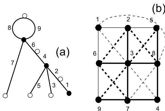
Figure 1. The dessin d’enfant (a) arising from the first subgroup of index 9 of the Kleinian group K^{(4)} and the Hesse configuration (b) that it stabilizes. The configuration consists of the union of a 3 \times 3 grid (plain lines) and another one that is skewed to it (dotted lines). Non-straight lines are not all drawn. The coordinatization is in terms of coset representatives of the subgroup K^{(4)} in the free group G as follows: 1 = e , 2 = y , 3 = yx , 4 = yx^{-1} , 5 = yx^2 , 6 = yx^{-1}y , 7 = yx^{-1}yx , 8 = (yx^{-1})^2 , 9 = yx^{-1}yx^2 . Only the thin lines (passing through e ) have their cosets mutually commuting.
