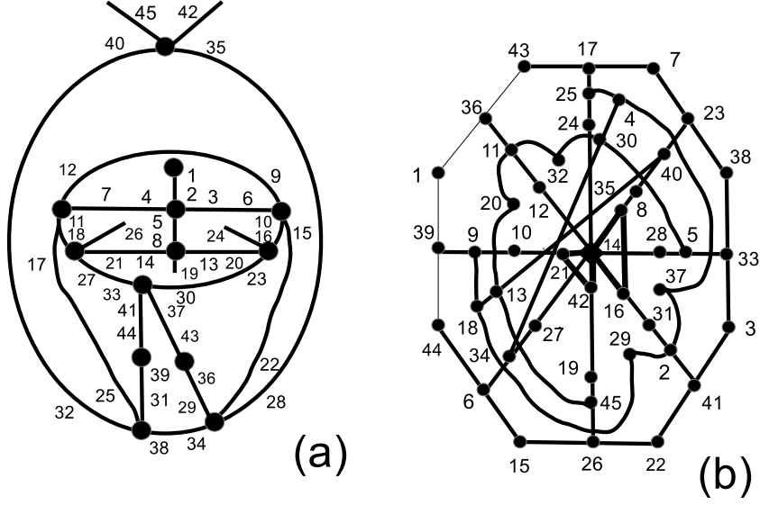
Figure 7. The dessin in (a) arising from the unique subgroup of index 45 isomorphic to A_6 of the Kleinian group K^{(5)} (white points are implicit in the drawing). This dessin stabilizes the thin generalized octagon GO(2, 1) shown in (b). The vertices of the two thicker triangles at the center of the picture (b) form lines (8, 14, 16) and (14, 21, 42) . They share the point 14 (the big bullet) and the latter does not lie on either straight line around it. More precisely, there are three lines left along a straight segment going through the point 14 such as (6, 34, 27) , (27, 35, 8) and (8, 40, 23) . The list of coset representatives corresponding to the labeling 1 to 45 is [e, y, yx, yx^{-1}, yx^2, yxy, yx^{-1}y, yx^2y, (yx)^2, yxyx^{-1}, yx^{-1}yx, (yx^{-1})^2, yx^2yx, yx^2yx^{-1}, yxyx^2, yxyx^{-1}y, yx^{-1}yx^2, yx^{-1}yxy, (yx^2)^2, yx^2yxy, yx^2yx^{-1}y, yxyx^2y, yxyx^{-1}yx, yxyx^{-1}yx^{-1}, yx^{-1}yx^2y, yx^{-1}yxyx, yx^{-1}yxyx^{-1}, yxyx^2yx, yxyx^2yx^{-1}, yxyx^{-1}yxy, yx^{-1}yx^2yx, yx^{-1}yx^2yx^{-1}, yx^{-1}yxyx^{-1}y, yxyx^2yx^2, yxyx^2yxy, yxyx^2yx^{-1}y, yxyx^{-1}yxyx, yx^{-1}yx^2yx^2, yx^{-1}yx^2yxy, yx^{-1}yx^2yx^{-1}y, yx^{-1}yxyx^{-1}yx^{-1}, yxyx^2yxyx^{-1}, yxyx^2yx^{-1}yx, yx^{-1}yx^2yxyx, yx^{-1}yx^2yx^{-1}yx] . As in previous diagrams, thick lines have non-commuting cosets.
