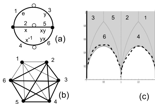
Figure 4. The dessin in (a) arising from the congruence subgroup of index 6 of type \Gamma(2) of the Kleinian group K^{(1)} . This dessin stabilizes the (maximally contextual) complete graph K_6 shown in (b). The thick line corresponds to non-commuting cosets. The corresponding polygon \Gamma(2) is shown in (c).
