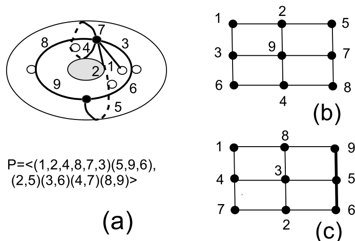
Figure 3. The dessin d'enfant (a) arising from the subgroup of index 9 and permutation group \mathbb{Z}_3^2 \rtimes \mathbb{Z}_2^2 in the Kleinian group K^{(19)} . This dessin stabilizes the non-contextual grid (b) from the stabilizer subgroup \mathbb{Z}_1 and the contextual one (c) from the stabilizer subgroup \mathbb{Z}_2 . The list of coset representatives corresponding to the labeling [1, 2, \dots, 9] is as follows [e, x, x^{-1}, x^2, xy, x^{-1}y, x^{-2}, x^3, xyx] . The thick line corresponds to non-commuting cosets.
