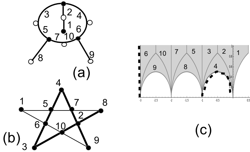
Figure 5. The dessin in (a) arises from the unique subgroup of index 10 of the Kleinian group K^{(1)} isomorphic to S_5 . This dessin stabilizes Mermin's pentagram shown in (b). As it is modular the dessin can also be seen as a tiling of the upper-half plane in (c). The list of coset representatives corresponding to the labelling [1, 2, \dots, 10] is [e, y, yx, yx^{-1}, yxy, yx^{-1}y, (yx)^2, yxyx^{-1}, yx^{-1}yx, (yx^{-1})^2] . The thick lines of (b) correspond to non-commuting cosets.
