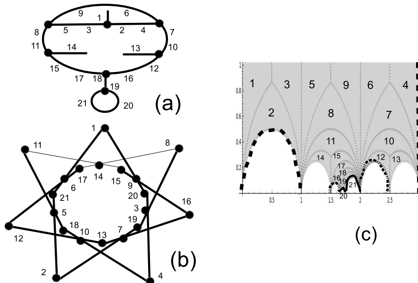
Figure 6. The dessin in (a) arises from the unique subgroup of index 21 of the Kleinian group K^{(1)} isomorphic to SL(2, 7) (white points are implicit in the drawing). This dessin stabilizes the thin generalized hexagon GH(2, 1) shown in (b). As it is modular, the dessin can also be seen as a tiling of the upper-half plane in (c). The list of coset representatives corresponding to the labelling 1 to 21 is [e, x, x^{-1}, xy, x^{-1}y, xyx, xyx^{-1}, y^x, x^{-1}yx^{-1}, xyx^{-1}y, x^{-1}yxy, xyx^{-1}yx, xyx^{-1}yx^{-1}, x^{-1}(yx)^2, x^{-1}yxyx^{-1}, xyx^{-1}yxy, x^{-1}yxyx^{-1}y, xyx^{-1}(yx)^2, xyx^{-1}(yx)^2y, xyx^{-1}(yx)^3, xyx^{-1}(yx)^2yx^{-1}] . The thick lines of (b) correspond to non-commuting cosets.
