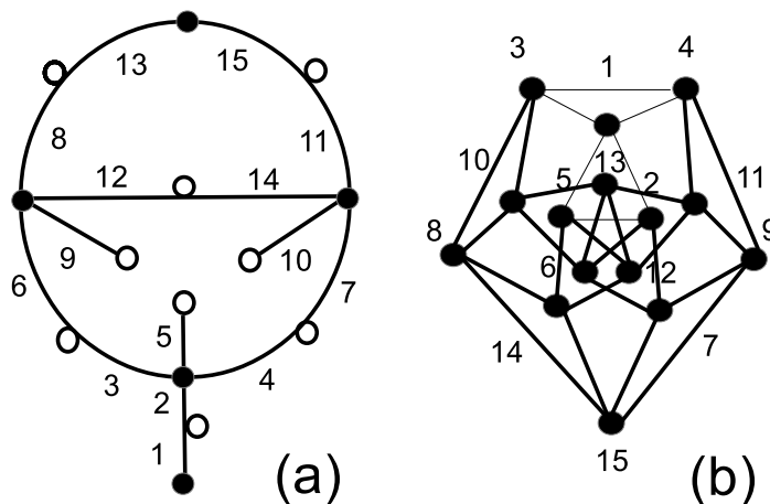
Figure 2. The dessin d'enfant (a) arising from the first subgroup of index 15 of the Kleinian group K^{(4)} and the line graph of the Petersen graph (b) that it stabilizes. The list of coset representatives corresponding to the labelling \{1, 2, \dots, 15\} is as follows [e, y, yx, yx^{-1}, yx^2, yxy, yx^{-1}y, (yx)^2, yxyx^{-1}, yx^{-1}yx, (yx^{-1})^2, yxyx^2, yxyx^{-1}y, yx^{-1}yx^2, yx^{-1}yxy] . Only the thin triangles (passing through e ) have their cosets mutually commuting.
