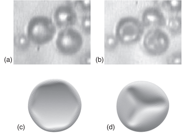
FIG. 8. Top: Snapshots from high-speed recordings of an encapsulated polymer/albumin at two moments during an acoustic cycle: (a) in the inflated state, and (b) in buckled state with wrinkles. Bottom: Numerical simulation of a fully deflated shell \Delta V/V = 0.759 (c) and a shell under re-inflation \Delta V/V = 0.234 (d). The shell has a relative thickness d/R = 3/\sqrt{7} = 0.0385 .
