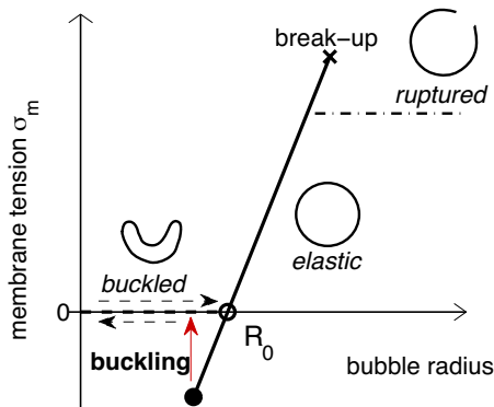
FIG. 4. Model for the shell membrane tension under large volume variation. As soon as the surface tension is negative enough to reach the buckling value (full circle), buckling occurs (large arrow) and the membrane tension vanishes (thick dashed line). The elastic state is recovered when the volume gets back to its rest value (open circle). When the rupture point is reached (cross), membrane tension saturates to the water value (dash dotted).
