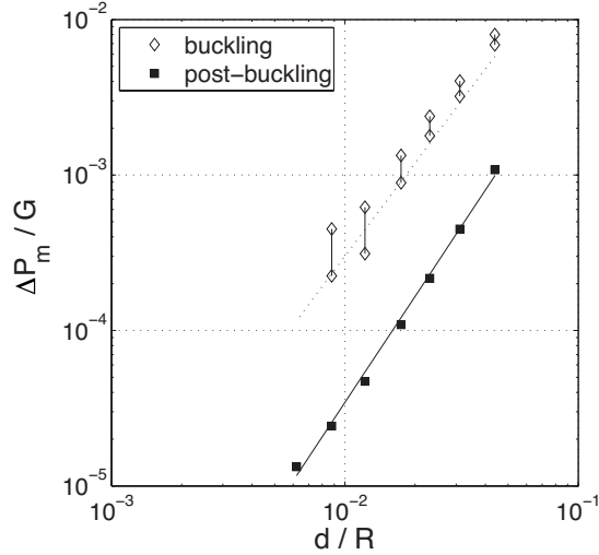
FIG. 2. Simulation results for the post-buckling pressure \Delta P_m^{\text{post-buckling}} (squares), evaluated in the plateau region of Fig. 1d, as a function of the relative shell thickness. The continuous line stands for a power-law fit with \Delta P_m^{\text{post-buckling}}/G = 1.193 \times (d/R)^{2.27 \pm 0.06} . The value of the exponent is in total agreement with theoretical predictions of post-buckling pressure derived in Appendix B. For comparison, we also plot the buckling pressure \Delta P_m^b from simulations (diamonds giving the range where simulation value is located), and the theoretical prediction (dashed line) from Eq. 7.
