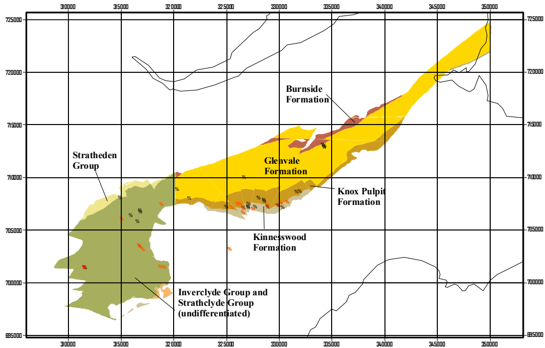
Figure 5 Location of known groundwater boreholes in the Upper Devonian/Lower Carboniferous aquifer in Fife
