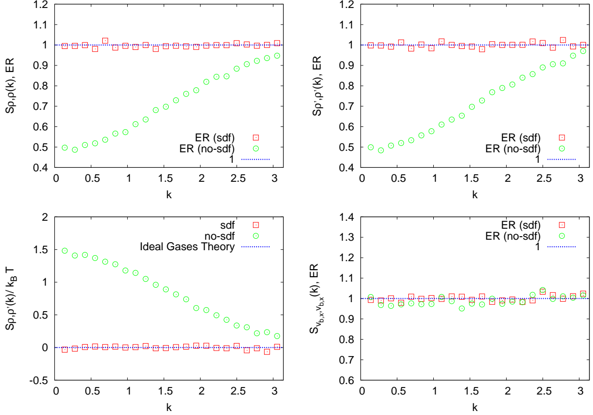
FIG. 2: Equilibrium ratio (ER) for the densities and the baricentric velocity as a function of wavevector magnitude k . Simulation results are normalized according to the theoretical predictions of Eqs. (79) and (82), except for the cross-density correlation, S_{\rho,\rho'}(k) = \langle \delta\hat{\rho}(k)\delta\hat{\rho}'(-k') \rangle , which is normalized by k_B T . The mutual interaction strength in Eq. (113) is set to \mathcal{G} = 0 in all the numerical simulations (ideal gases). To appreciate the effects of the noise on the momentum modes (see the first two equations in (100)), we repeated the numerical simulations by setting such noise to zero, i.e. without stochastic diffusion fluxes (no-sdf).
