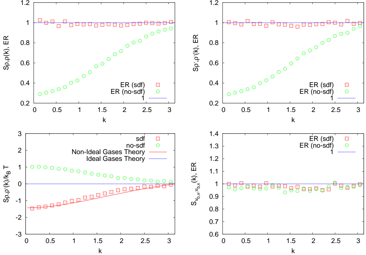
FIG. 3: Equilibrium ratio (ER) for the densities and the baricentric velocity as a function of wavevector magnitude k . Simulation results are normalized according to the theoretical predictions of Eqs. (79) and (82), except for the cross-density correlation, S_{\rho, \rho'}(k) = \langle \delta \hat{\rho}(k) \delta \hat{\rho}'(-k') \rangle , which is normalized by k_B T . The mutual interaction strength in Eq. (113) is set to \mathcal{G} = 0.4 in all the numerical simulations. For the simulation parameters chosen (see text for details), the critical point for phase separation is found at \mathcal{G}_c = 1.0 lbu. To appreciate the effects of the noise on the momentum modes (see the first two equations in (100)), we repeated the numerical simulations by setting such noise to zero, i.e. without stochastic diffusion fluxes (no-sdf).
