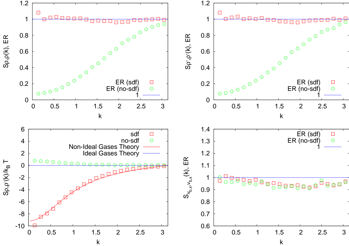
FIG. 4: Equilibrium ratio (ER) for the densities and the baricentric velocity as a function of wavevector magnitude k . Simulation results are normalized according to the theoretical predictions of Eqs. (79) and (82), except for the cross-density correlation, S_{\rho, \rho'}(k) = \langle \delta \hat{\rho}(k) \delta \hat{\rho}'(-k') \rangle , which is normalized by k_B T . The mutual interaction strength in Eq. (113) is set to \mathcal{G} = 0.85 in all the numerical simulations. For the simulation parameters chosen (see text for details), the critical point for phase separation is found at \mathcal{G}_c = 1.0 lbu. To appreciate the effects of the noise on the momentum modes (see the first two equations in (100)), we repeated the numerical simulations by setting such noise to zero, i.e. without stochastic diffusion fluxes (no-sdf).
