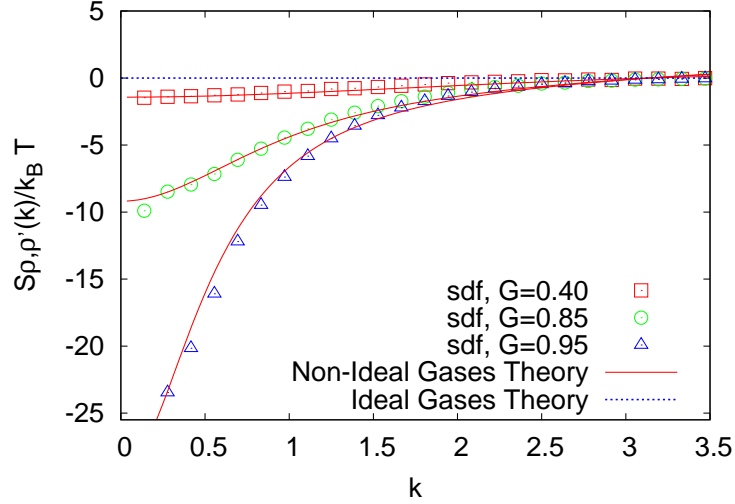
FIG. 5: The cross-density correlation S_{\rho,\rho'}(k) = \langle \delta \hat{\rho}(k) \delta \hat{\rho}'(-k') \rangle normalized by k_B T is reported as a function of the wavevector magnitude k . The mutual interaction strength in Eq. (113) is set to \mathcal{G} = 0.4 (squares), \mathcal{G} = 0.85 (circles), \mathcal{G} = 0.95 (triangles). Other simulation parameters are given in the text. The critical point for phase separation is found at \mathcal{G}_c = 1.0 lbu. All the numerical simulations are performed with the noise on the momentum modes, i.e. with stochastic diffusion fluxes (sdf), according to Eqs. (100). The theoretical prediction of the rhs of Eq. (82) is also reported (red solid line). Correspondingly, we also show the prediction for the ideal-gases ( \mathcal{G} = 0 ) case (blue dotted line).
