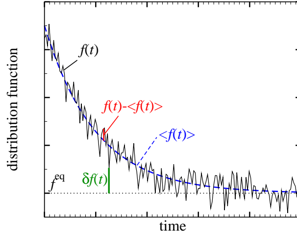
FIG. 1: A schematic view of the fluctuating Boltzmann distribution f(t) , its ensemble average \langle f(t) \rangle and its deviation from the equilibrium distribution f^{\text{eq}} . Note that, per definition, the equilibrium distribution function neither has any explicit time dependence nor exhibits any fluctuations. The ensemble averaged distribution function, \langle f(t) \rangle , on the other hand, is per construction free of fluctuations but may depend on time if the system is brought out of equilibrium by some perturbation. Since \langle f(t) \rangle converges towards f^{\text{eq}} for long times, the difference \delta f(t) = f(t) - f^{\text{eq}} becomes identical to f(t) - \langle f(t) \rangle asymptotically for t \rightarrow \infty .
