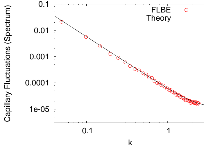
FIG. 6: Capillary fluctuations of a planar one-dimensional interface obtained with mean-field lattice interactions (see Sec. VII B). The equal-time spectrum of interfacial height fluctuations obtained from LBE simulations (circles) is compared with the theoretical structure factor (solid line) reported in Eq. (117). The wavevector in the interface region is indicated with k . Simulation parameters are reported in the text.
