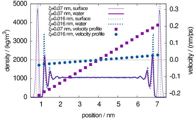
Fig. 3 Left axis: The density distribution of tethered atoms (thin lines) and water molecules (thick lines) in the random quenched case at \xi \simeq 0.07 nm (solid) and \xi \simeq 0.016 nm (dashed). Right axis: water velocity profiles at shear rate \dot{\gamma} \simeq 0.016\text{ps}^{-1} (squares: \xi \simeq 0.07 nm; circles: \xi \simeq 0.016 nm).
