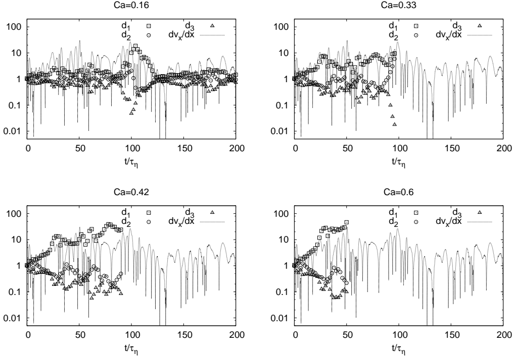
FIGURE 2. Time signals of the square-root of the eigenvalues, d_1(t) (= [\lambda_m^{(1)}]^{1/2}) , d_2(t) and d_3(t) in logarithmic units obtained from solving the Maffettone & Minale droplet model coupled to Lagrangian time history of turbulent velocity gradients from DNS at Re_\lambda = 185 . We also superpose the time history of |A_{11}(t)| , the absolute value of one component of the velocity gradient tensor (solid line).
