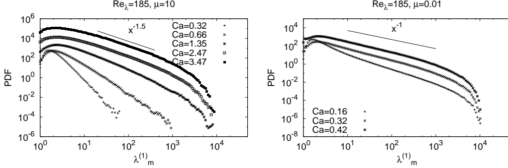
FIGURE 12. Left panel: PDF of the largest eigenvalue of the morphology tensor for various Capillary numbers, for viscosity ratio \mu = 10 . Note that the straight line has a slope -1.5 and that the saturation of the tails happens at a higher Ca value compared to the critical Capillary estimated by (6.1). Right panel: the same for \mu = 0.01 . Now the transition is very similar to the case \mu = 1 , and the tail has the -1 power law slope.
