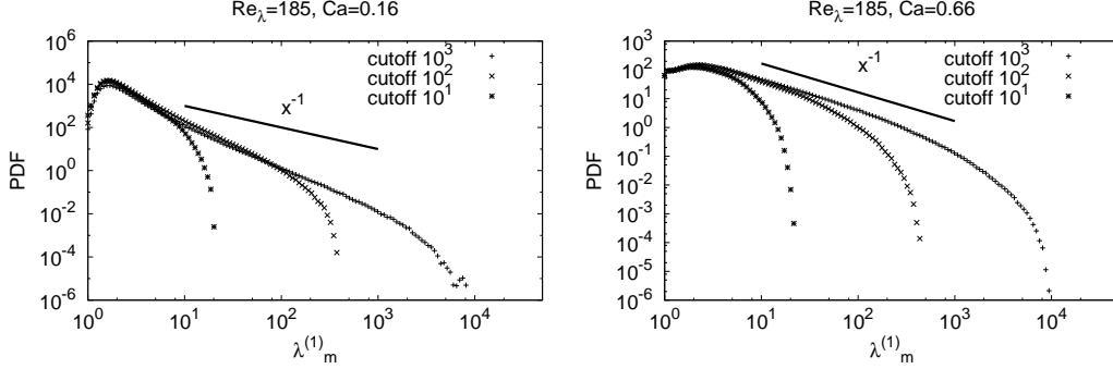
FIGURE 5. Probability density functions of largest eigenvalue \lambda_m^{(1)} of the morphology tensor \mathbf{M} , obtained from solving the Maffettone & Minale droplet model coupled to Lagrangian time history of turbulent velocity gradients from DNS at Re_\lambda = 185 . Different symbols denote different imposed cutoff values for the maximum deformation value d_1/d_3 = 10, 10^2, 10^3 . Results are shown for two Capillary numbers Ca = 0.16 below (left) and above (right) Ca_c . We also superpose the power law behaviour \propto x^{-1} predicted for the saturation slope when Ca > Ca_c .
