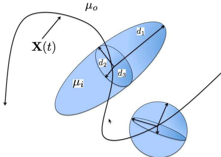
FIGURE 1. Typical ellipsoidal shape of one droplet along the turbulent trajectory. The droplet centre of mass \mathbf{X}(t) is supposed to follow the evolution of a fluid particle and the droplet deformation is governed by the statistics of the fluid velocity gradients along the trajectory, \partial_i u_j(\mathbf{X}(\mathbf{t}), t) . We denote by \mu_o the viscosity of the carrying fluid and by \mu_i that inside the droplet. The droplet is always assumed of ellipsoidal shape with the three semi-axes ordered as d_1 \geq d_2 \geq d_3 .
