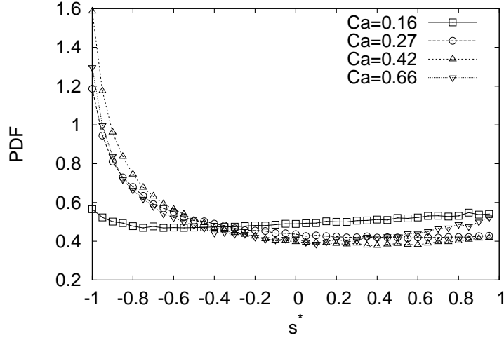
FIGURE 9. PDFs of s^* , for different Ca .
