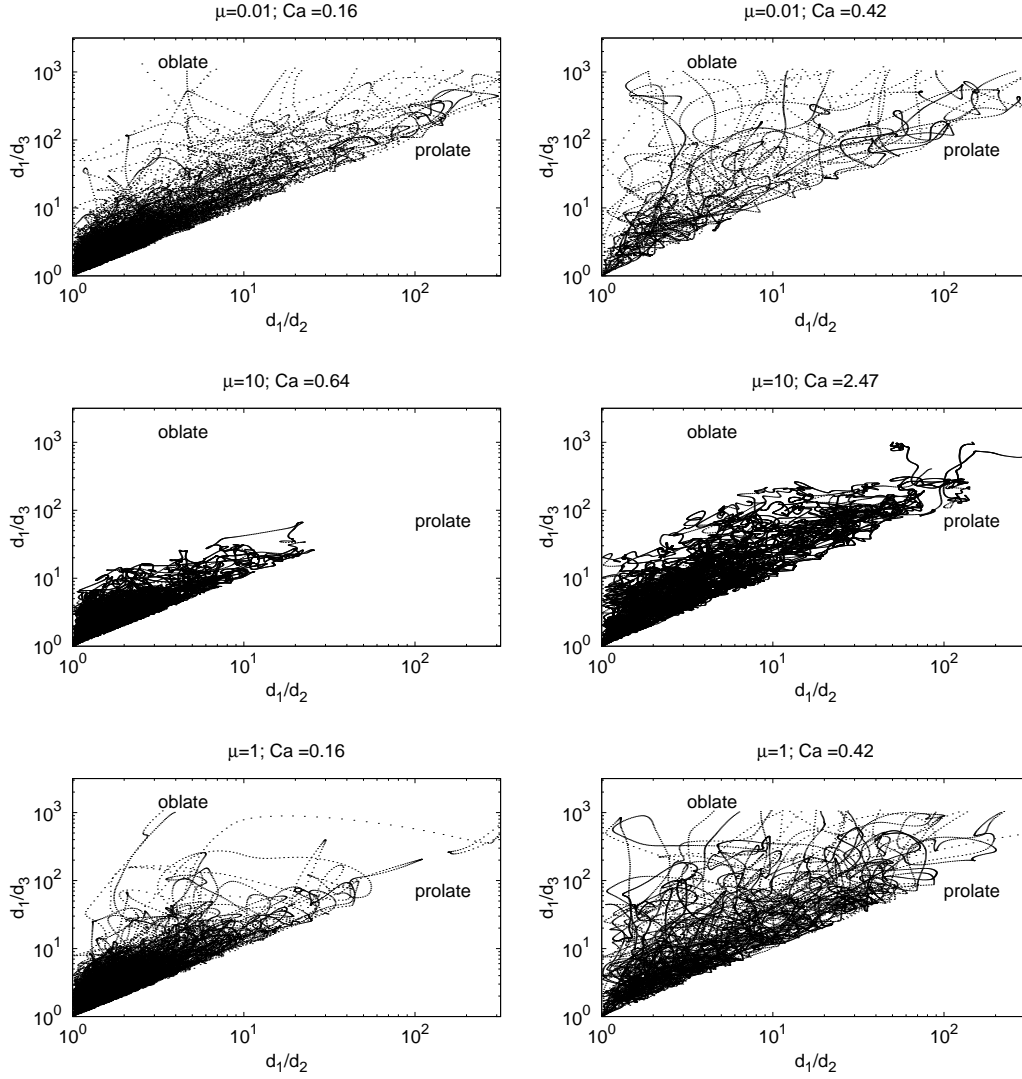
FIGURE 15. Scatter plot of ratio between ellipsoidal semi-axis sizes.
