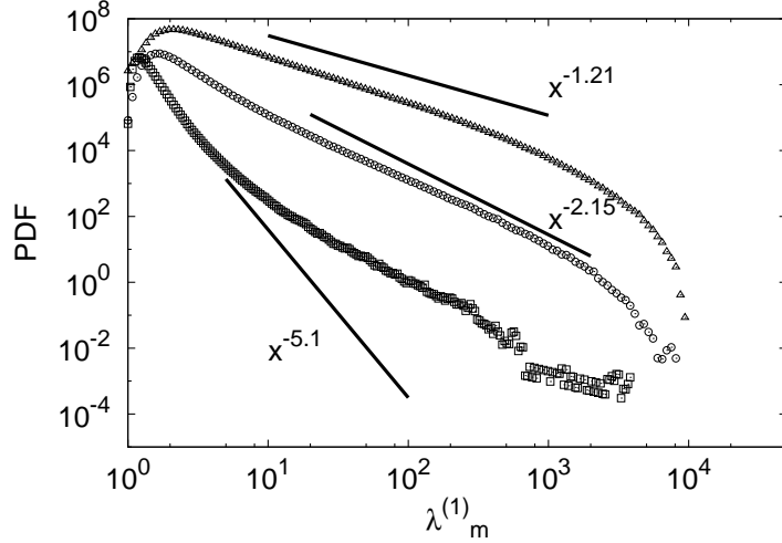
FIGURE 7. PDFs of the largest eigenvalue of the morphology tensor for Ca = 0.06 (squares), Ca = 0.16 (circles) and Ca = 0.33 (triangles) as computed from the simulation. The corresponding theoretical power law predictions are shown as solid lines with the predicted slopes (exponents) noted.
