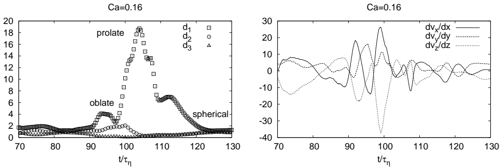
FIGURE 3. Left: Enlargement of the previous panel for Ca = 0.16 around the peak of the deformation of the droplet. Right: the corresponding evolution for the three diagonal entries of the velocity gradient tensor, A_{11}(t) , A_{22}(t) , A_{33}(t) .
