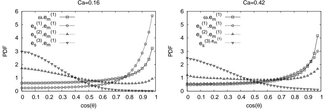
FIGURE 10. PDFs of cosine of angle between the particle's largest eigenvector, e_m^{(1)} , with vorticity and the three eigenvectors of \mathbf{S} , for two Ca (left and right).
