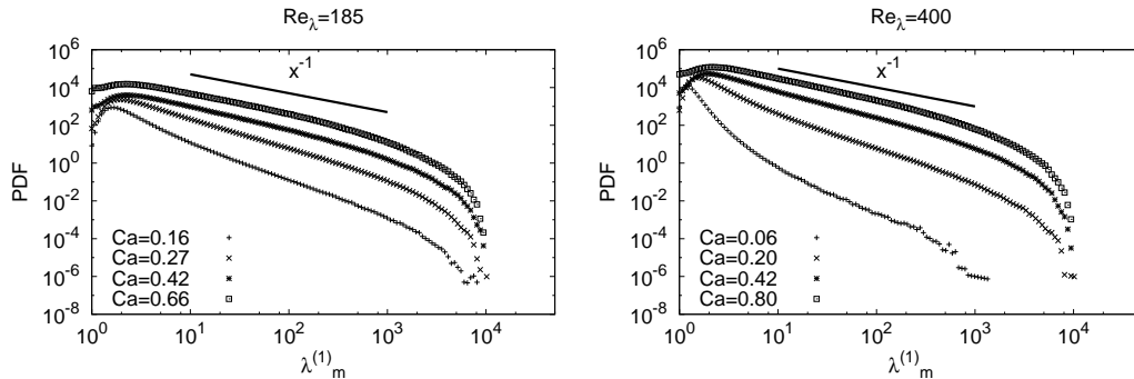
FIGURE 4. Probability density functions of largest eigenvalue \lambda_m^{(1)} of the morphology tensor \mathbf{M} , obtained from solving the Maffettone & Minale droplet model coupled to Lagrangian time history of turbulent velocity gradients from DNS at Re_\lambda = 185 (left) and Re_\lambda = 400 (right). Different curves correspond to different values of the capillary number, both below and above the critical value, Ca_c \sim 0.42 . The solid line represents the power law behaviour \propto x^{-1} . Curves are shifted vertically for the sake of presentation.
