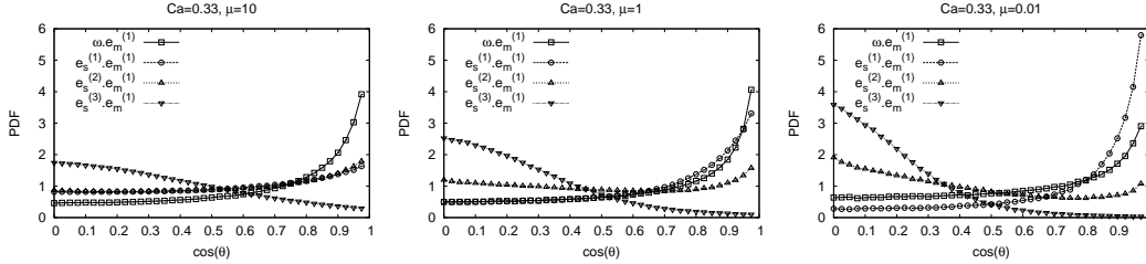
FIGURE 14. PDFs of cosine of angles. Comparison between alignment with vorticity and strain-rate eigendirections for three different viscosity ratios, at Ca = 0.33 .
