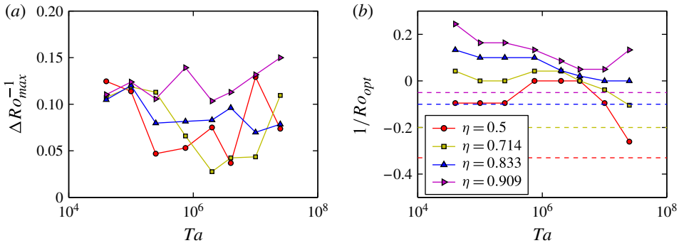
FIGURE 9. (Colour online) (a) The 95 % peak width \Delta Ro_{max}^{-1} versus Ta for the four values of \eta analysed in numerics. The peak width can be seen to vary with driving, and for smaller gaps is larger for larger values of Ta . (b) Plot of Ro_{opt}^{-1} versus Ta for the same four values of \eta . The location of the optimal transport has a very strong dependence on the driving, especially for the largest values of \eta . As driving increases beyond the numerically studied range and overlaps with experiments, Ro_{opt}^{-1} should tend to the experimentally found values, represented as dashed lines. The asymptote for \eta = 0.5 is obtained from Merbold et al. (2013). The trend appears to be less clear for \eta = 0.909 , but this might be understandable from the peak width at the highest driving Ta .
