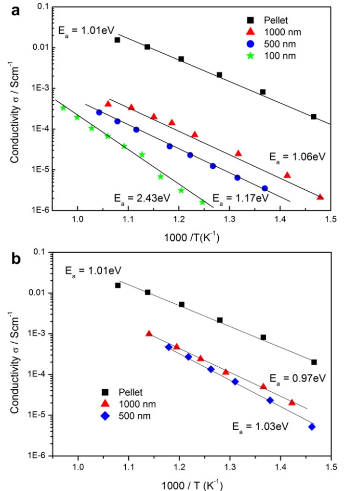
Fig. 8. Arrhenius plots of (a) LSGM/STO/MgO and (b) LSGM/NdGaO 3 films of different thicknesses together with LSGM pellet.
