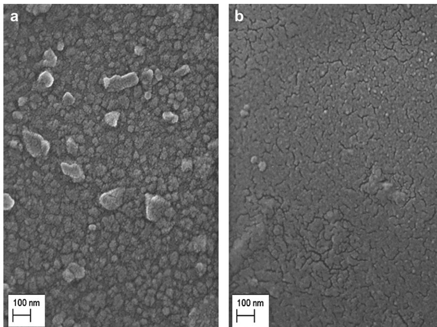
Fig. 4. SEM micrographs (top-view) of 1 μm thick (a) LSGM/STO/MgO and (b) LSGM/NdGaO 3 films.
