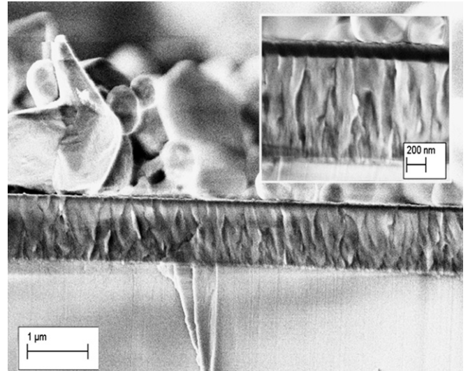
Fig. 7. FE-SEM micrograph (cross-section) of 1 μm thick LSGM/STO/MgO film.
