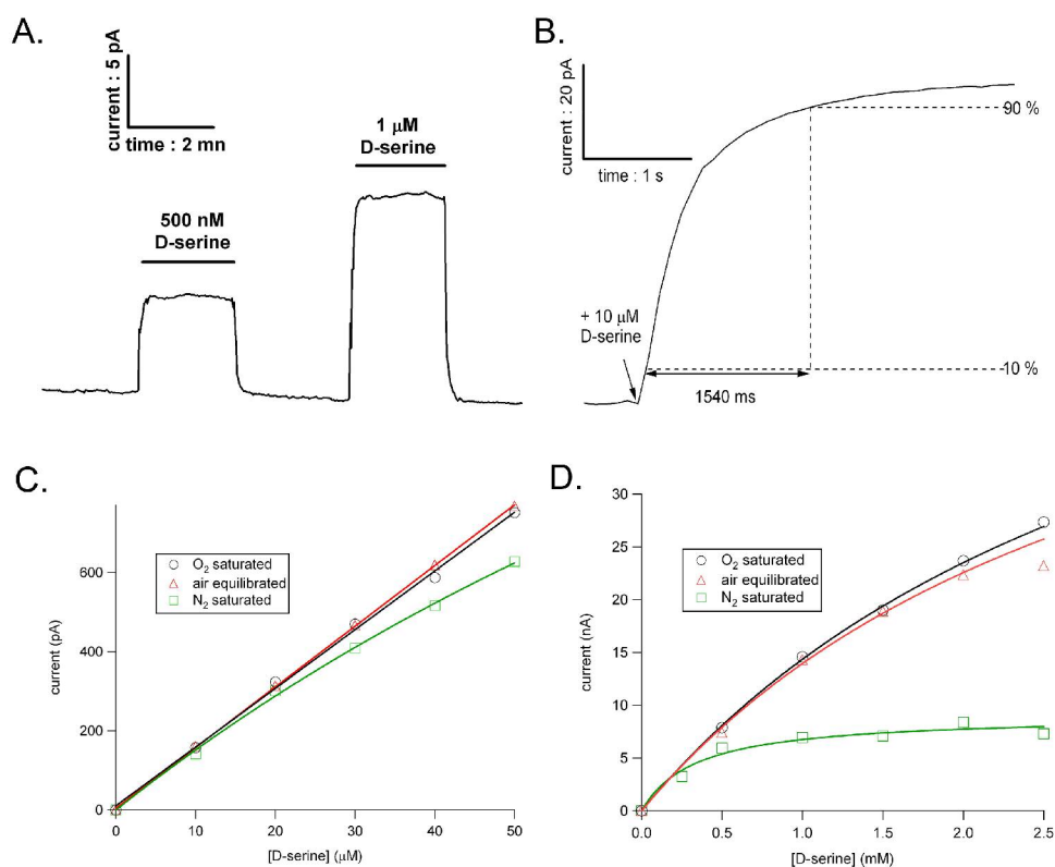
Figure 2: D-serine detection. A. Response of the biosensor to changes in D-serine concentration. The electrode was rapidly transferred from phosphate buffered saline (PBS) to a 500 nM or 1 μM D-serine solution and back to PBS. The change in D-serine concentration was detected as a step in the oxidation current recorded by the electrode. B. Response time. The electrode was switched from 0 to 10 μM D-serine. The response time was defined as the time between 10% and 90% of the current step. In order to obtain a higher time resolution, the signal was averaged over 10 ms (instead of 1 s). C. Calibration curves of a microbiosensor at three oxygen concentrations (N 2 -saturation, air equilibrated and O 2 -saturation) in the 0-50 μM D-serine concentration range. Except for the N 2 -saturated medium, the oxidation current shows a linear dependence on the D-serine concentration. D. Calibration curves of the microbiosensor in the 0-2.5 mM D-serine concentration range. The calibration was made in N 2 -saturated, in air equilibrated and in O 2 -saturated PBS. The relationship between the oxidation current and D-serine concentration fits with a classical Michaelis-Menten equation in which O 2 is not-limiting in catalysis.
