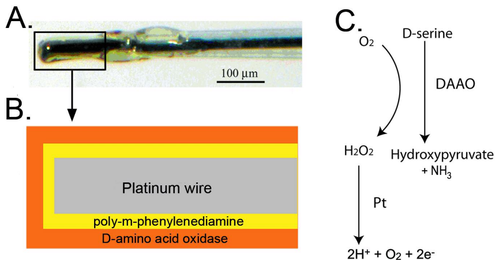
Figure 1: Design of the biosensor. A. Photomicrograph of the tip of a RgDAAO microbiosensor. The enzymatic layer appears as a translucent, yellow membrane. B. Schematic representation of the D-amino acid oxidase (RgDAAO) microbiosensor. A platinum wire is covered with a layer of poly-m-phenylenediamine (PPD) and an enzymatic membrane of RgDAAO. C. Enzymatic reaction allowing D-serine detection at the microbiosensor: D-serine is oxidized into hydroxypyruvate by RgDAAO with equimolar production of hydrogen peroxide ( \text{H}_2\text{O}_2 ) that diffuses through the PPD layer and is oxidized by the platinum wire. \text{H}_2\text{O}_2 oxidation gives rise to two electrons detected by the patch-clamp amplifier.
