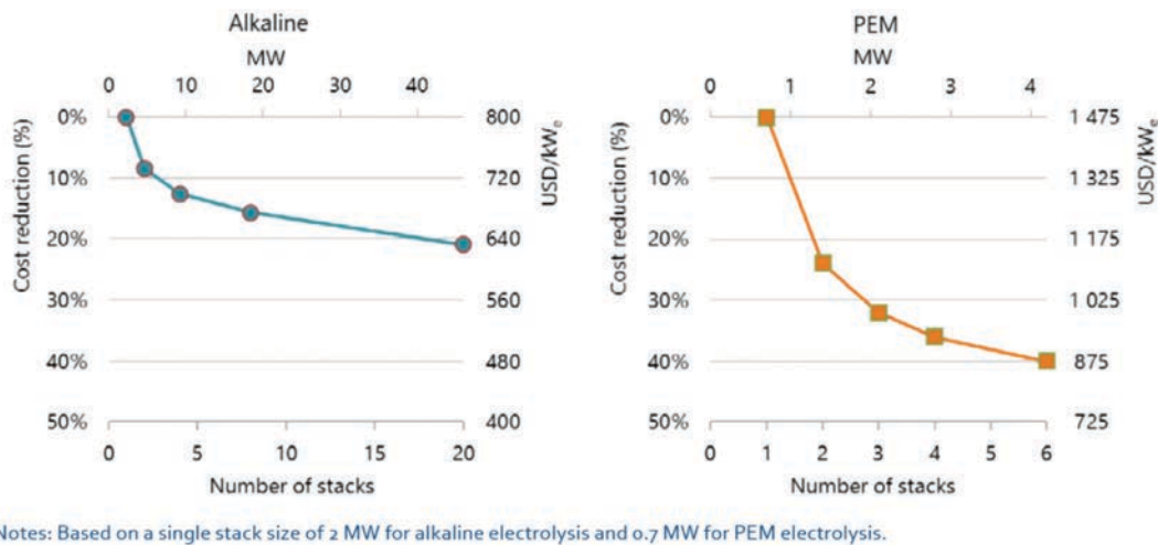
Fig. 168 Estimate of cost reduction associated with plant size increases for AWEs and PEMWEs. Reproduced from the IEA. 1889
