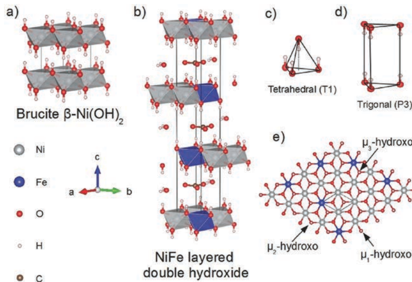
Fig. 50 Typical structure of Brucite type Ni(OH) 2 and hydrotalcite-like NiFe LDH. Reproduced with permission from ref. 812. Copyright Wiley 2016.
