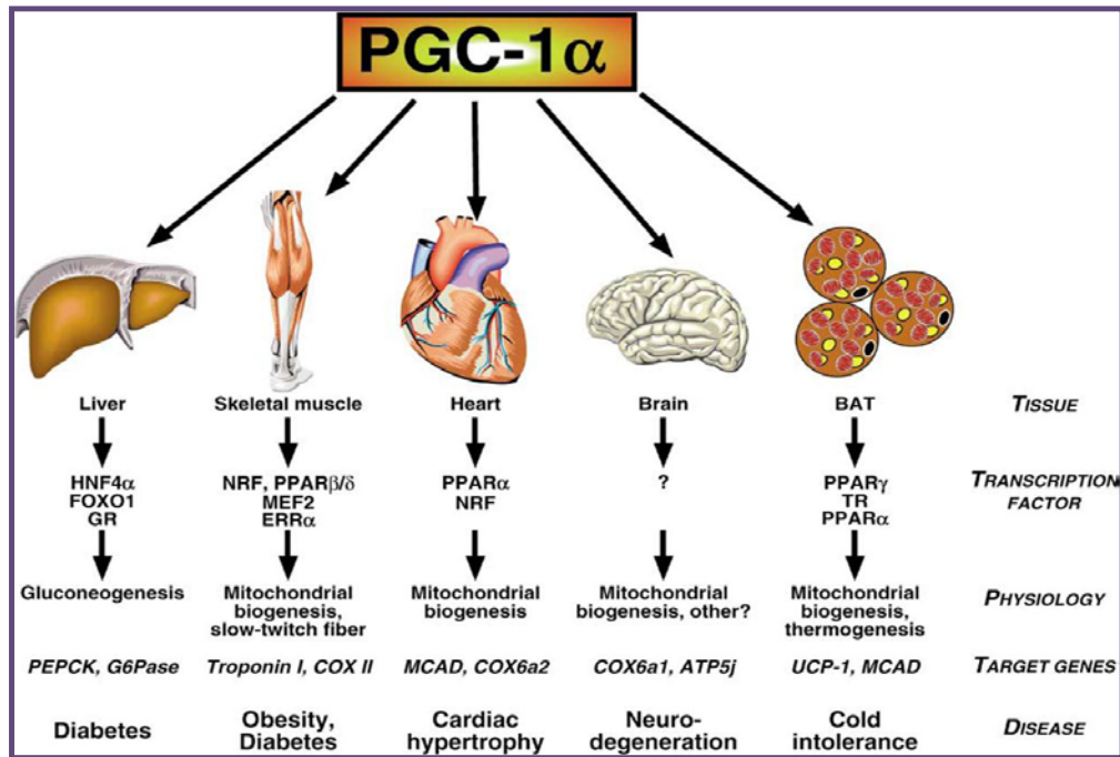
Fig. 6- Schematic representation of the different functions of PGC-1 \alpha in its target tissues.
