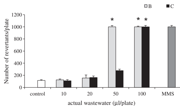
Fig. 6. Number of revertants/plate obtained after exposure to different amounts of actual wastewater B and C. Control, i.e. untreated bacteria. MMS: positive control, i.e. bacteria treated with methyl methane sulfonate (1 \mu\text{g/plate} ). Results from three experiments \pm S.D. are presented. * p < 0.0001 vs. control, according to the Student's t test.
