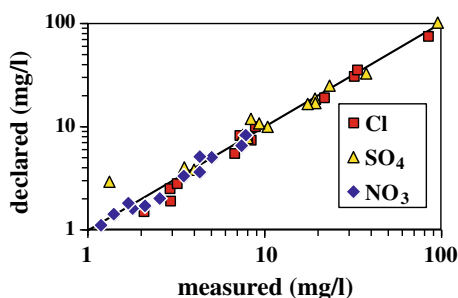
Fig. 4 Binary correlation diagrams of measured vs. declared in the label values of chloride, sulphate and nitrate in the analysed bottled water samples. The line represents the 1/1 ratio
