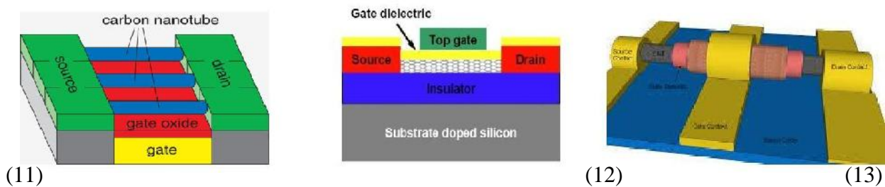
[fig 11, fig 12 and fig 13 show the back gated, top gated and wrap gated CNTFET structure respectively [6]]
