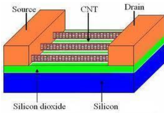
[ fig10 shows the structure of CNTFET[5]]
