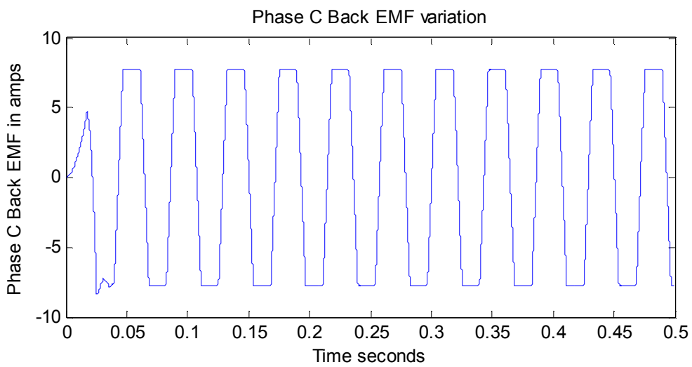
Fig.6.5: Phase Back EMF s variation of Motor
