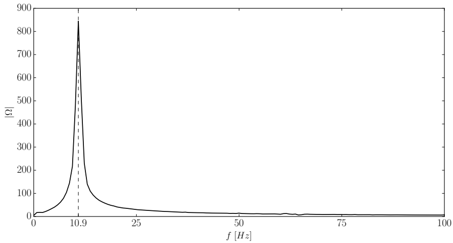
Figure 3. A discrete FFT of a time series y_m(t) of the pendulum’s linear displacement acquired from the measurement of angle \varphi on the experimental stand. One dominant frequency is found as marked by the dashed line.
