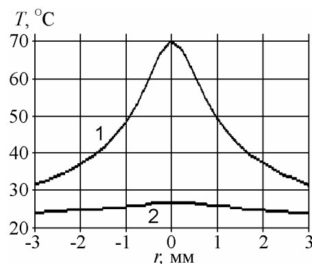
Fig. 3. Medium temperature profile
