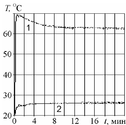
Fig. 4. Dependence of medium temperature in beam centre on time
