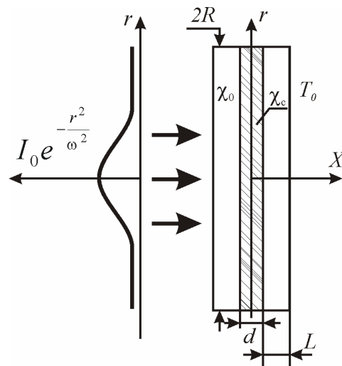
Fig. 1. For calculation of thermodiffusion bleaching of two-component medium in thin-layer cylindrical cell
