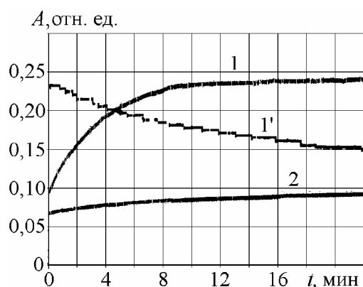
Fig. 2. Dependence of cell transmission coefficient (beam diameter is 1 mm, power 60 mWt) on time, cell wall thickness: 1) 2,25, 2) 0,125 mm, (1') is the transmission coefficient reduction at beam power increasing in 20 times
