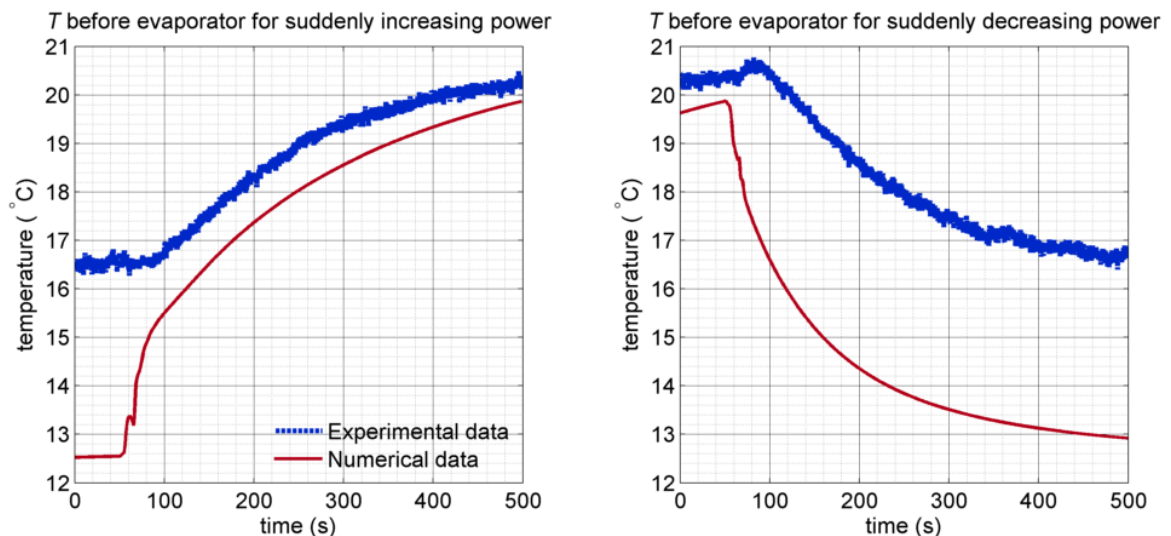
Figure 16 Liquid temperature before the evaporator
