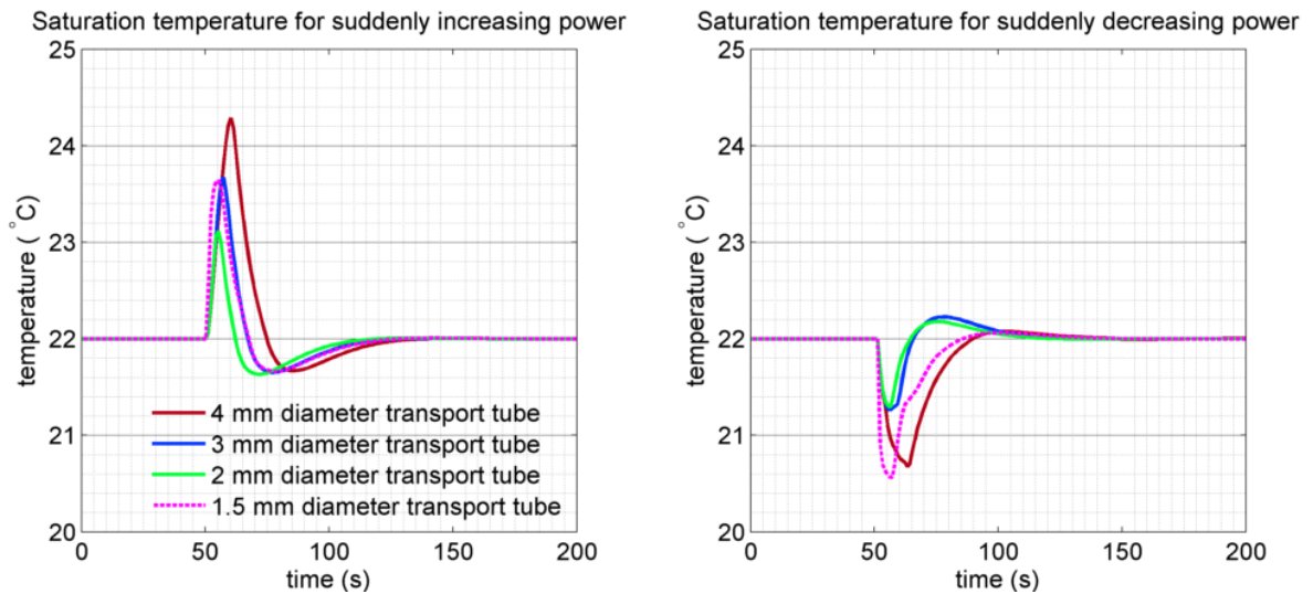
Figure 17 Saturation temperature in the evaporator for different transport tube diameters
