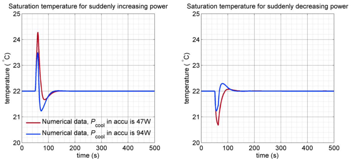
Figure 18 Calculated saturation temperature with 47W and 94W of cooling power in the accumulator
