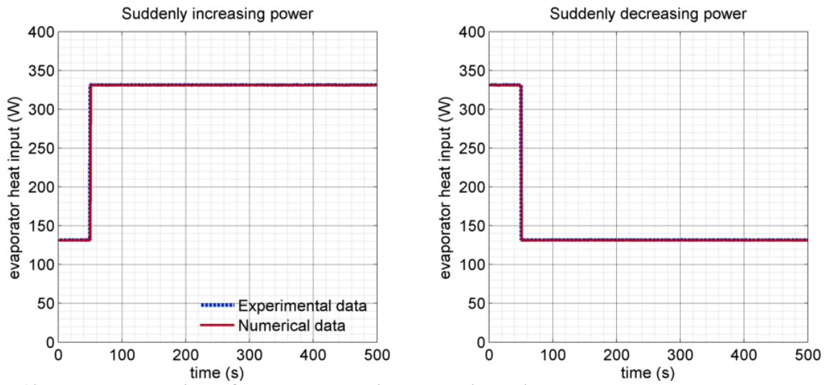
Figure 12 Evaporator heat input for both the experiment and simulation
