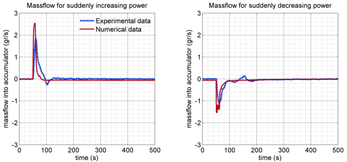
Figure 13 Massflow into the accumulator as a result of an increase and decrease of the heat input
