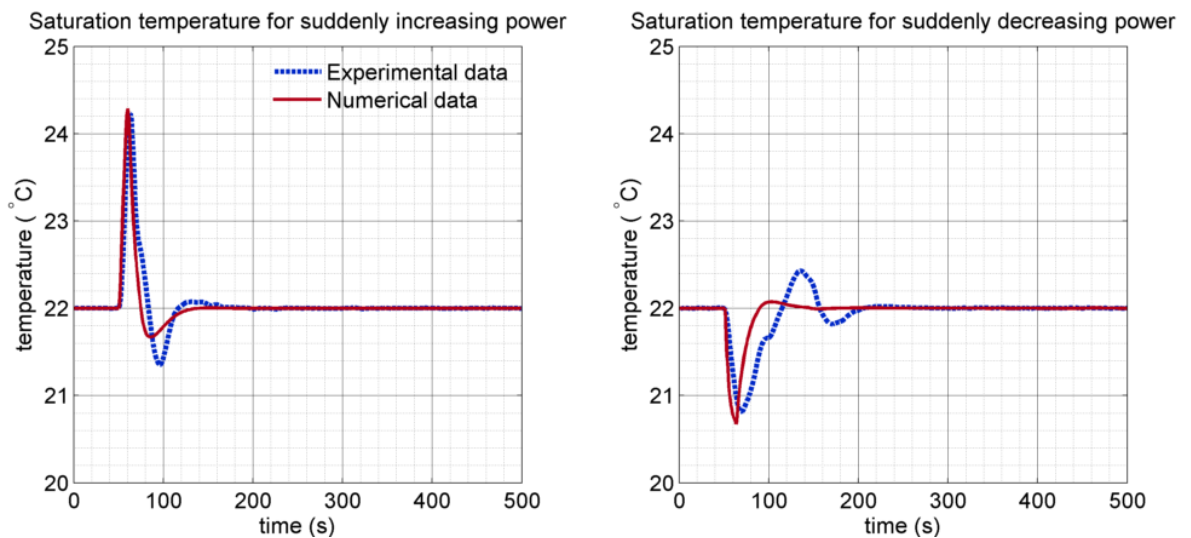
Figure 14 Saturation temperature after the evaporator
