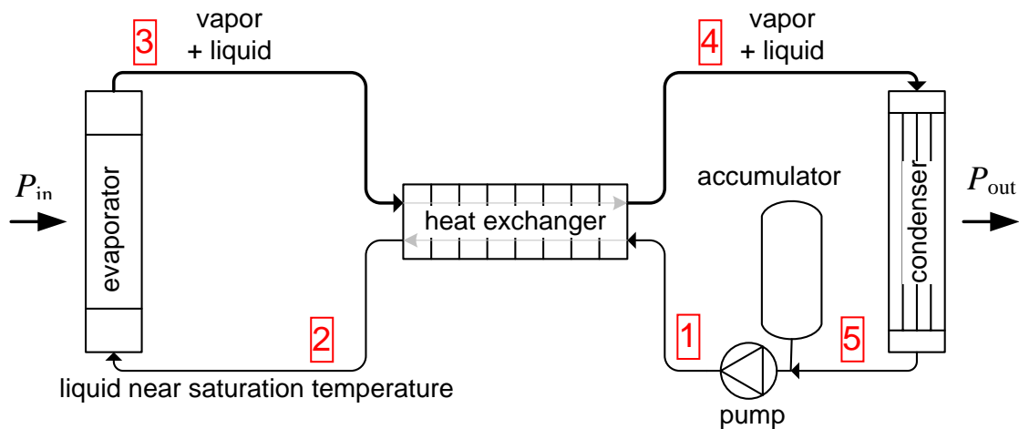
Figure 1 Schematic drawing of a 2 \Phi -MPFL with heat exchanger. The red numbers 1 to 5 correspond to the numbers in the pressure-enthalpy diagram in Figure 3
