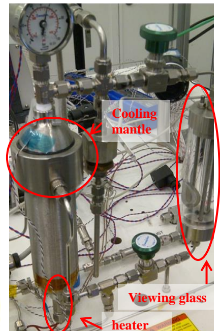
Figure 10 Photo of the accumulator
