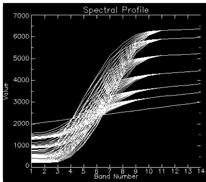
Figure1. Effects of leaf chlorophyll and LAI on canopy reflectance in the red edge
