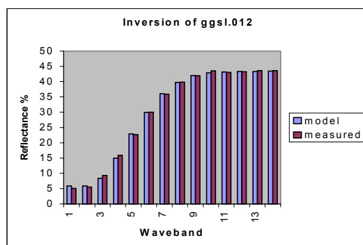
Figure 2. Measured and modelled hyperspectral reflectance data for a model inversion.
