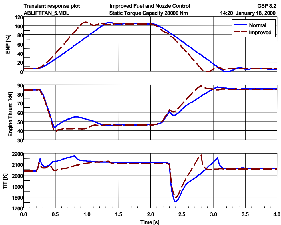
Figure 15 : Lift-fan (dis)engagement response with faster nozzle actuator and lower max. accel fuel
