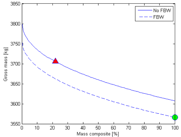
Figure 6 Minimum helicopter mass (green circle) is found for 100% composite mass in the fuselage and a fly-by-wire flight control system
