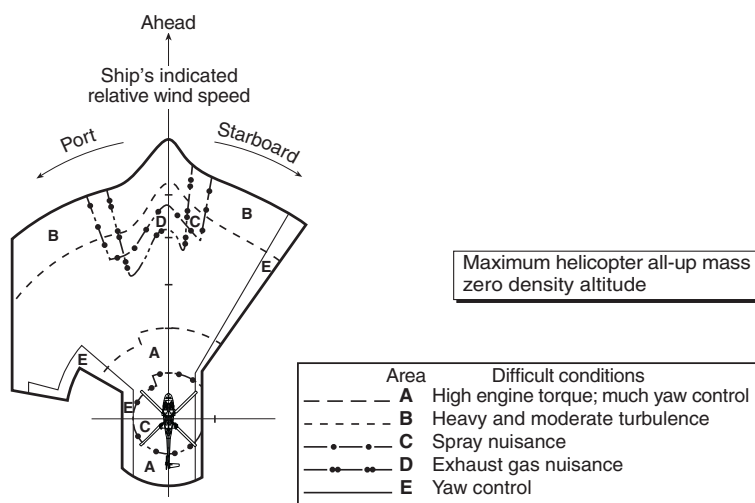
Figure 16 Candidate Flight Envelope, for fore/aft take-off and landing, corrected for ship anemometer system information.
