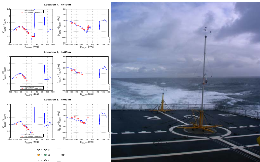
Figure 7 NLR moveable measuring masts on flight deck. The graphs on the left show the comparison of wind-tunnel- and full-scale measurement results.
