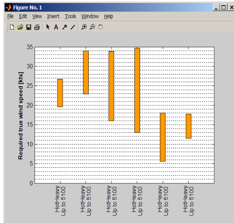
Figure 18 Graphic display to present true wind speed required for helicopter-ship flight trials.
