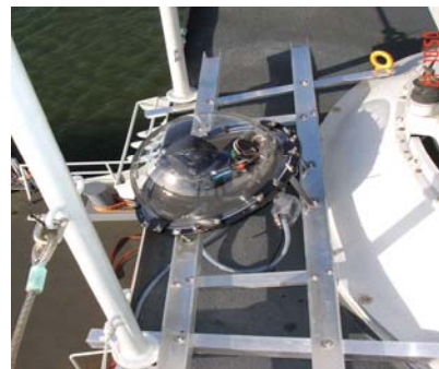
Figure 28 External installation of the video camera.
