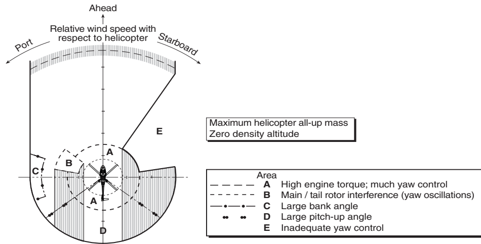
Figure 11 Detailed results from land based hover trials.
