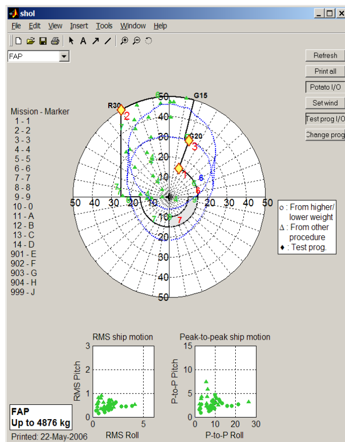
Figure 17 MATLAB™ Graphical User Interface in use with helicopter flight trials on board a ship.
