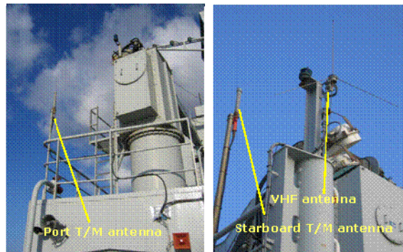
Figure 26 NLR telemetry - and VHF antenna as installed on a ship.
