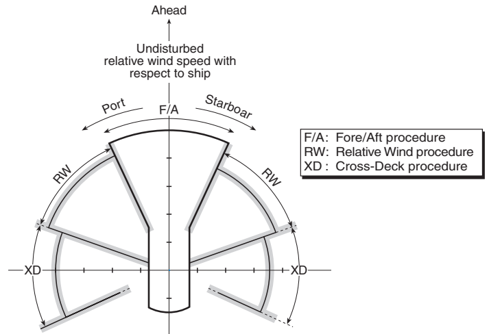
Figure 15 Example of a resultant Candidate Flight Envelope.
