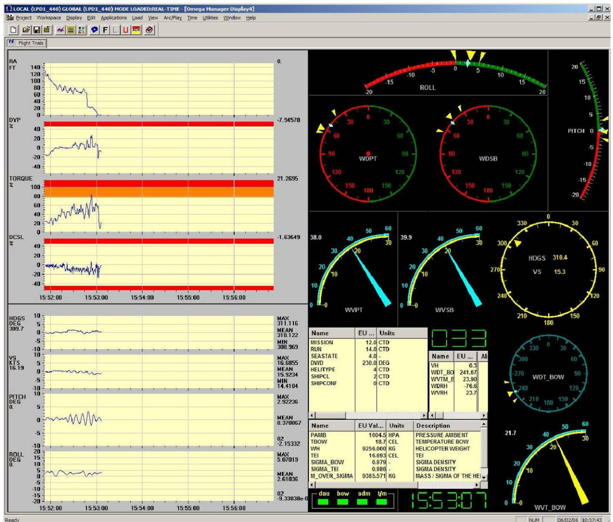
Figure 19 Real-time Quick-Look display for flight trials.
