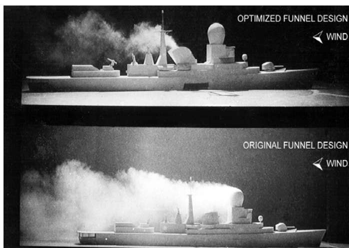
Figure 6 Stack & exhaust gas nuisance investigation on a wind tunnel model.
