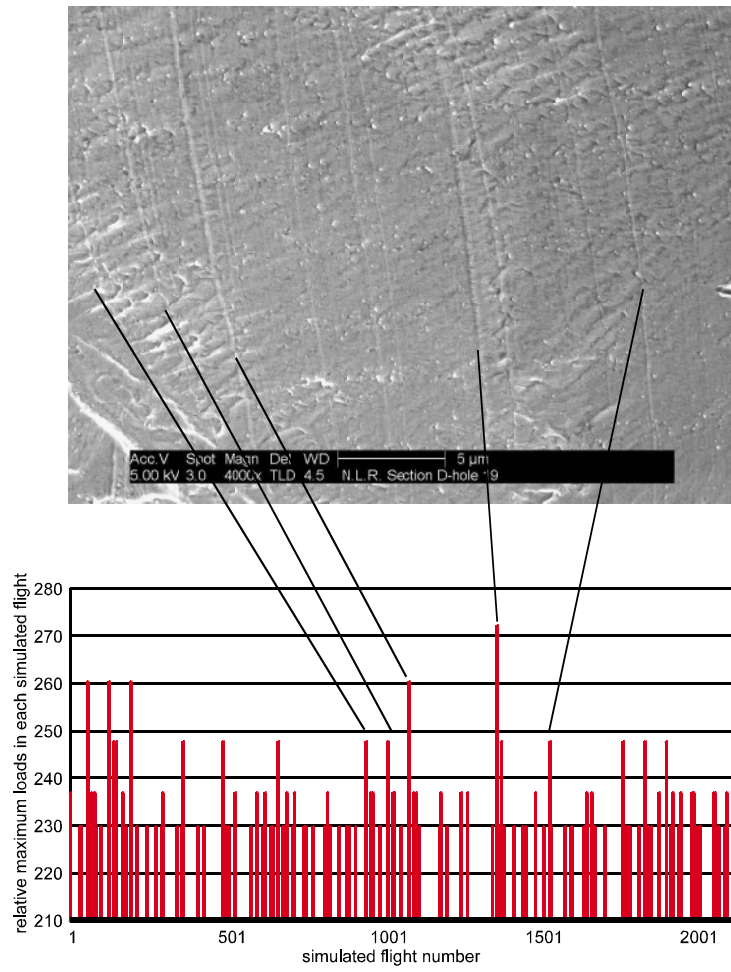
Fig. 5 Example identification of severe flights from crack front markings by peak loads
