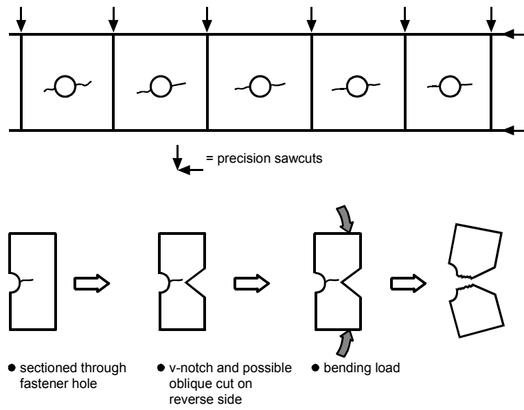
Fig. 3 Procedure for opening up cracks
