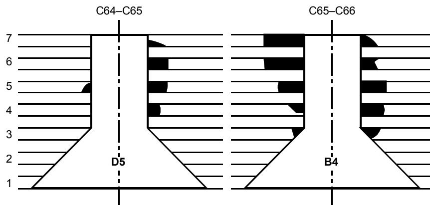
Fig. 4 Examples of GLARE cracking
