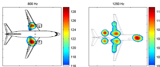
Figure 6: Typical noise source maps of a noisy aircraft (left, engines dominate) and a quiet aircraft (right, also airframe sources contribute).
