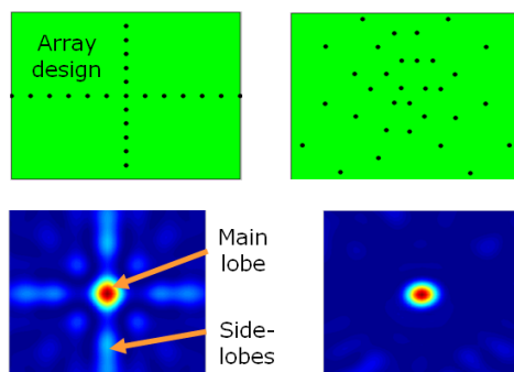
Figure 13: Effect of the array design on the side lobes, both for a cross-shaped array and a sparse array.
