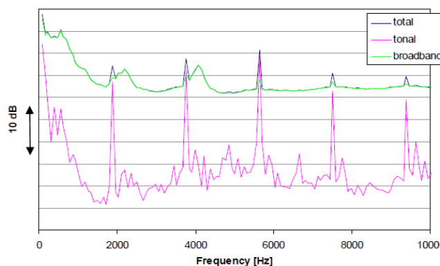
Figure 11: Average auto-spectrum at microphone array in Figure 10, + breakdown into tonal and broadband noise.
