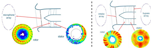
Figure 12: Beamforming results on rotor and stator with mode detection arrays in the intake (left) and both in the intake and bypass duct (right).
