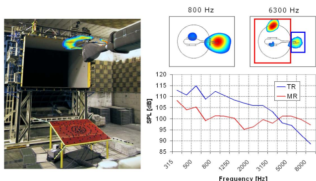
Figure 8: Helicopter test in DNW-LLF, including source spectra of tail (TR) and main rotor (MR), determined with source integration over the surfaces, indicated by the red and blue rectangles.
