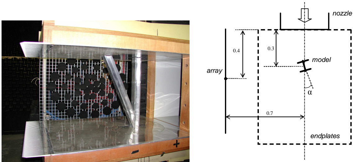
Figure 1: KAT test section with microphone array and bluff body (picture and top view, dimensions in m).
