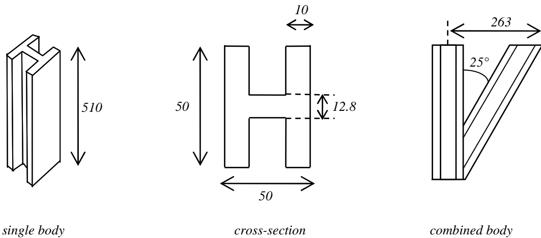
Figure 2: Lay-out of bluff bodies (dimensions in mm).
