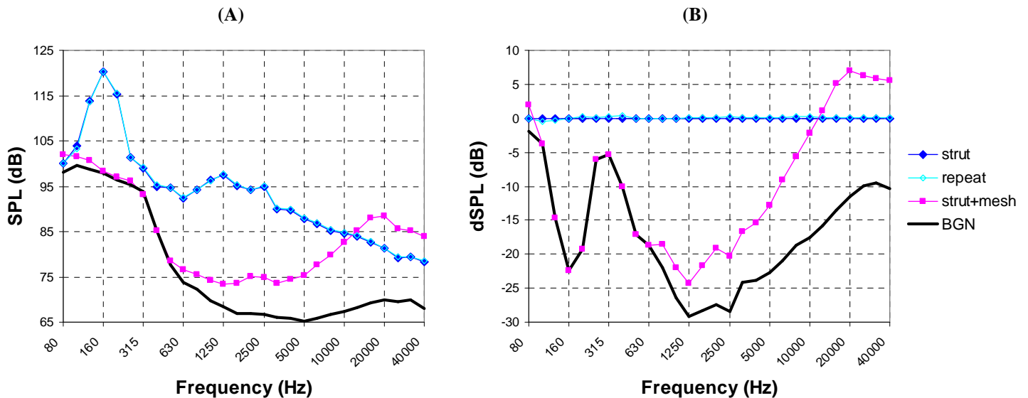
Figure 5: (A) Repeatability and signal-to-noise ratio for single strut with and without mesh (70 m/s; \alpha=0^\circ ). (B) Representation of mesh effect in terms of relative sound levels.
