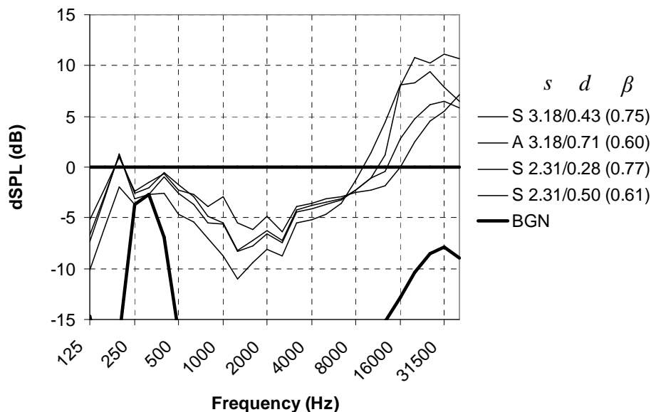
Figure 9: Effect of wire diameter d and mesh width s (indicated in mm) for circular steel (“S”) and aluminum (“A”) meshes on the single strut (70 m/s; \alpha=0^\circ ). The porosity \beta for each mesh is indicated in parentheses.
