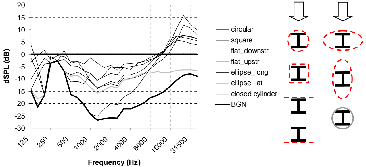
Figure 10: Effect of mesh shape for aluminum meshes on single strut ( s=2.54 mm; d=0.64 mm; 70 m/s; \alpha=0^\circ ).
