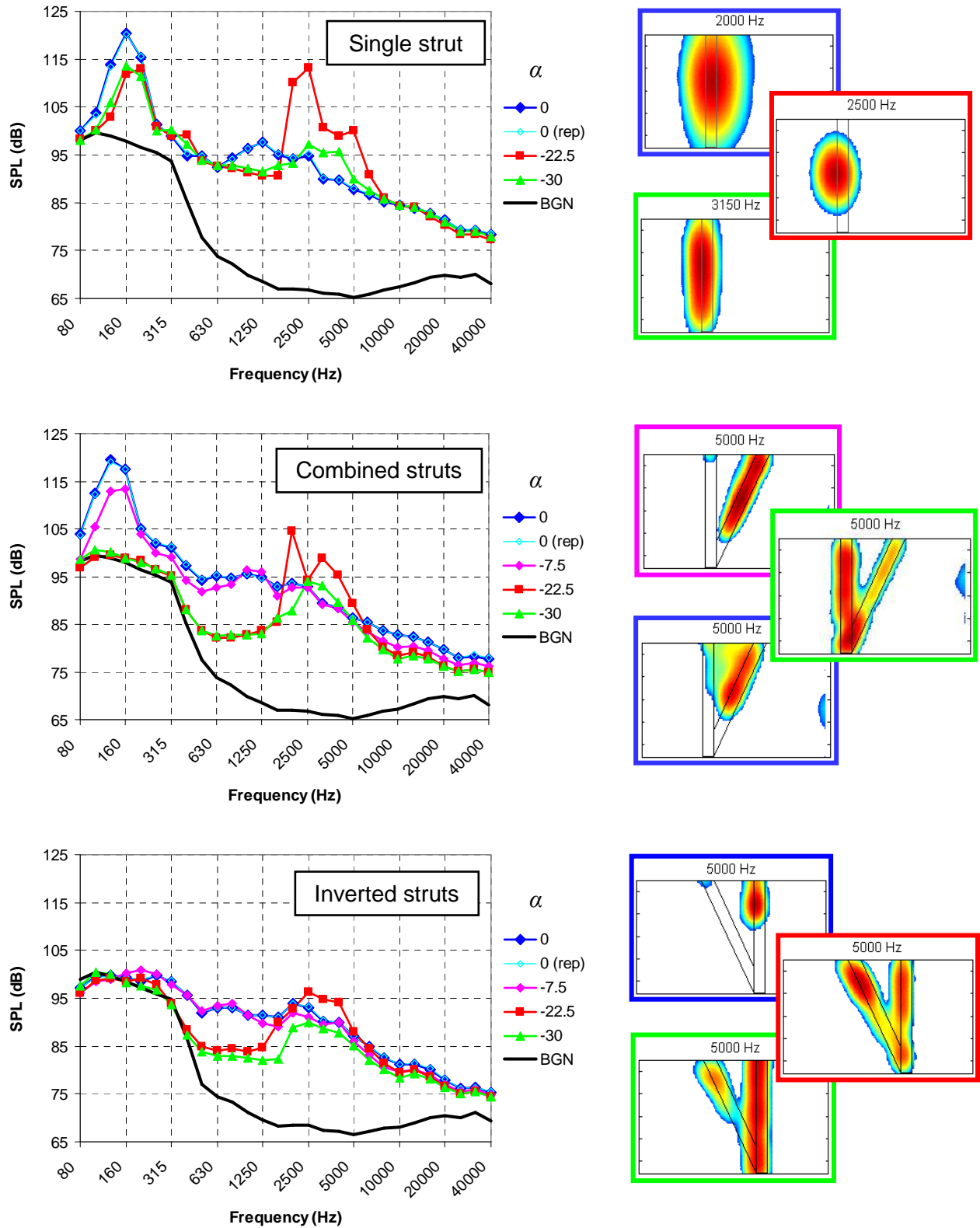
Figure 6: Baseline noise from single, combined, and inverted struts, with illustrative source maps (70 m/s). The legend indicates the angles of attack selected for the mesh assessment.
