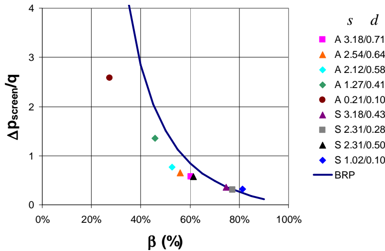
Figure 14: Flow resistance of isolated aluminum and steel meshes as a function of porosity.
