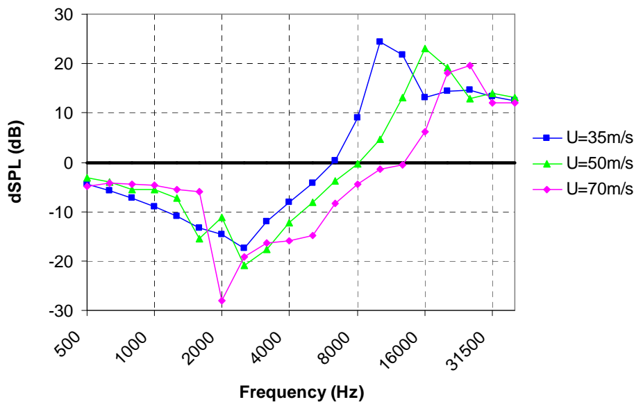
Figure 8: Effect of flow speed on high-frequency noise for circular aluminum mesh on single strut ( s=2.12 mm; d=0.58 mm; \alpha=-22.5^\circ ).
