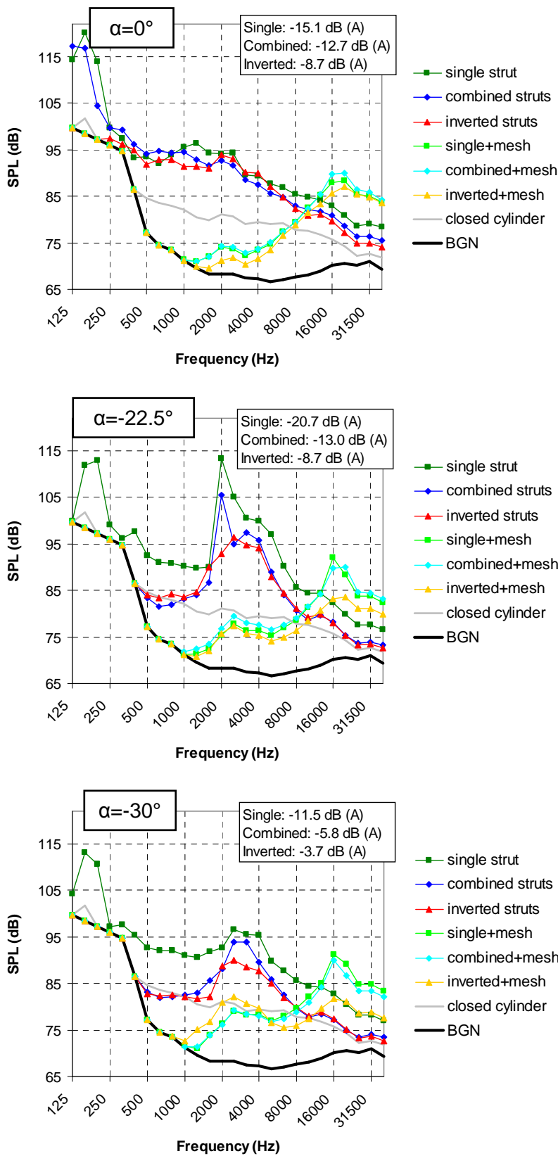
Figure 13: Acoustic effect of meshes for different models at different angles of attack (70 m/s).
