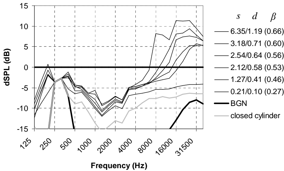
Figure 7: Effect of wire diameter d and mesh width s (indicated in mm) for circular aluminum meshes on the single strut (70 m/s; \alpha=0^\circ ). The porosity \beta for each mesh is indicated in parentheses.
