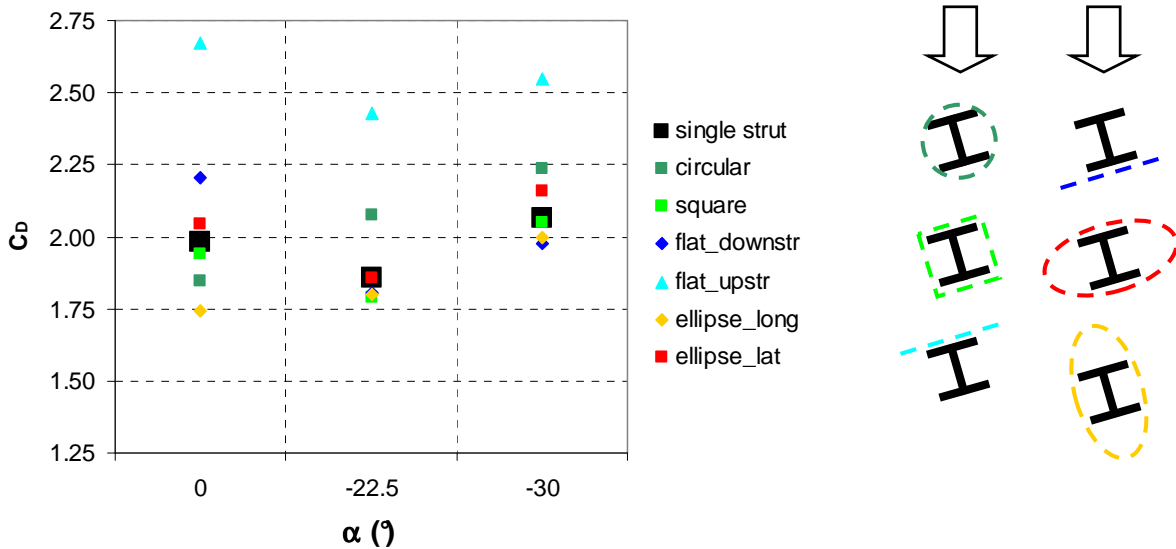
Figure 16: Flow resistance for different mesh shapes on single H-strut (70 m/s).
