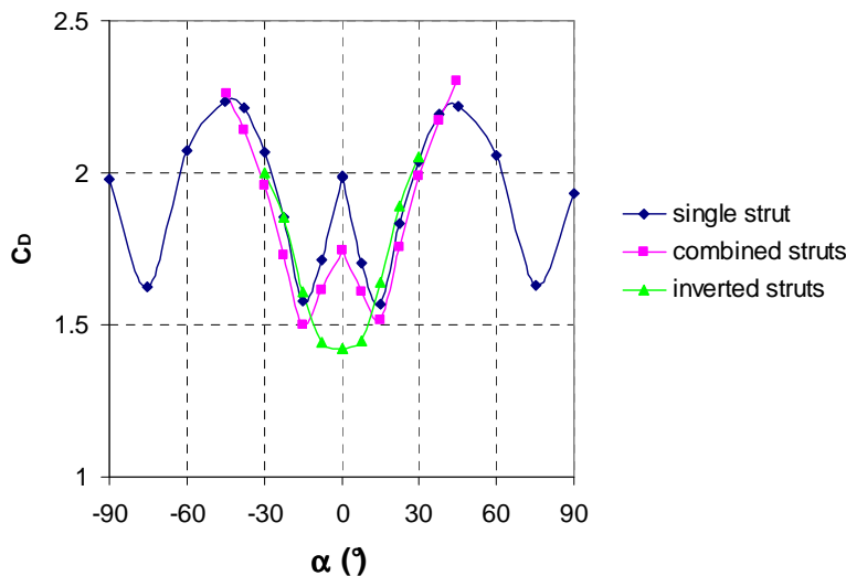
Figure 15: Flow resistance of baseline models as a function of angle of attack (70 m/s).
