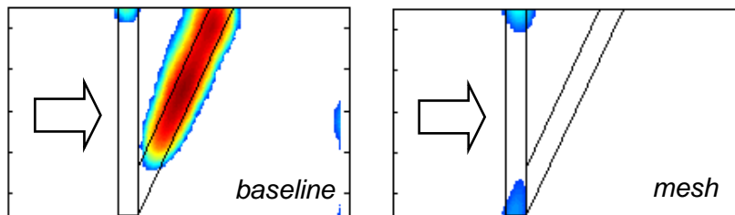
Figure 12: Example source maps showing effect of lateral elliptic mesh on upstream component (5 kHz; 70 m/s; \alpha=-7.5^\circ ).
