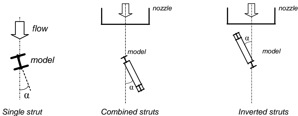
Figure 4: Definition of angle of attack for different models.
