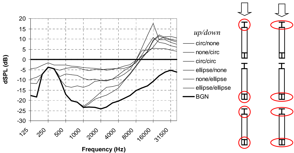
Figure 11: Effect of aluminum meshes on the combined struts ( 70 m/s; \alpha=0^\circ ). The legend indicates which mesh was mounted to the up- and downstream struts.
