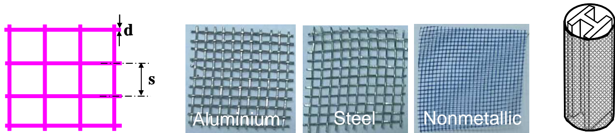
Figure 3: Definition of mesh dimensions, example pictures of materials, and installation on the H-strut.
