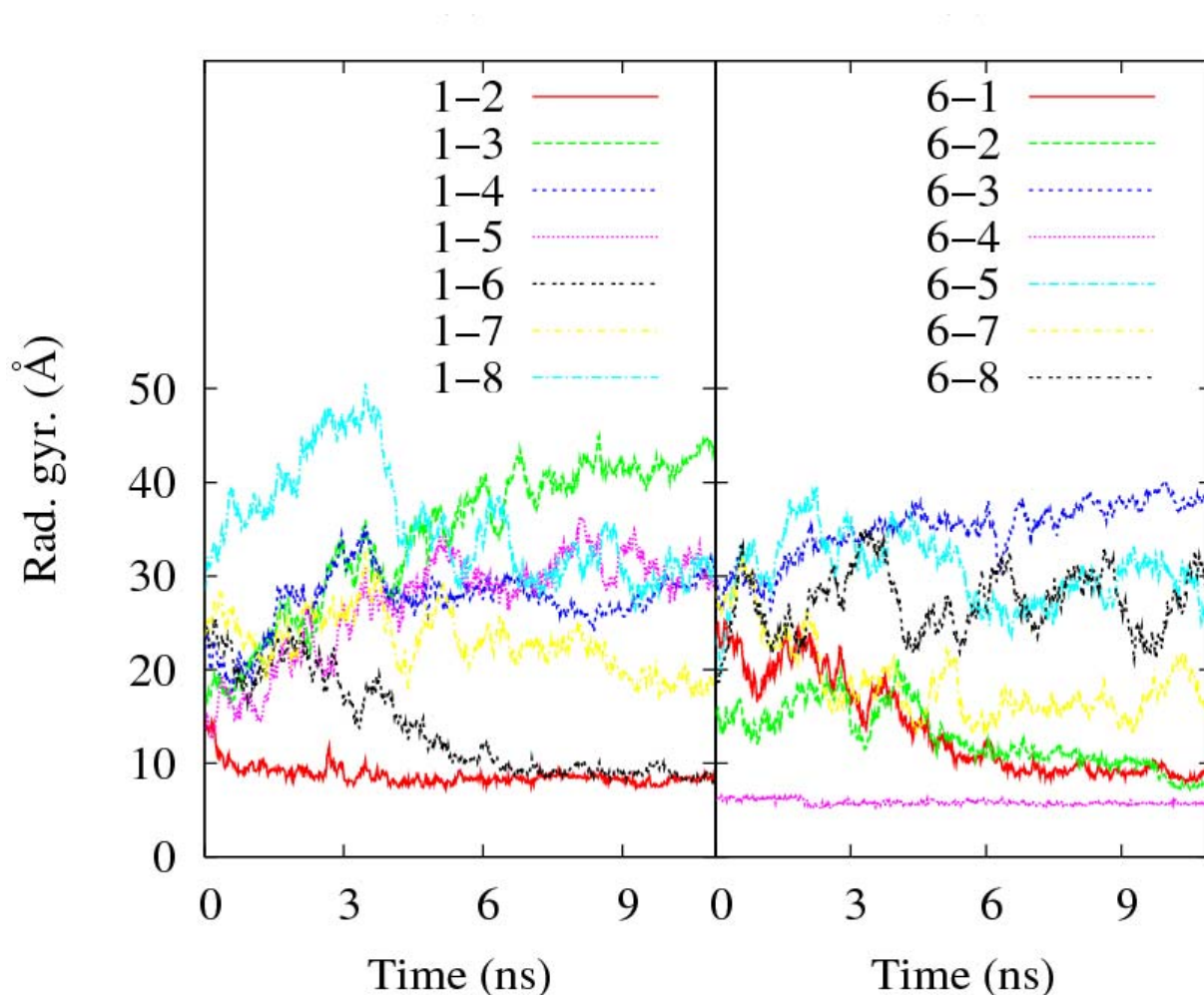
FIG. 10: Evolution of the radii of gyration during the simulation. Left panel – Radii of gyration of all pairs of molecules involving TNB1, The radii of gyration of pairs: TNB1-TNB2 and TNB1-TNB6 systematically decrease during the simulation. We identify three NOM fragments: TNB1, TNB2, and TNB6 that aggregate. Right panel – Evolution of the radii of gyration of all pairs of molecules involving TNB6. We can identify the four pairs of NOM fragments that aggregate during the last four picoseconds of the simulation: TNB1-TNB2, TNB1-TNB6, TNB6-TNB2, and TNB6-TNB4.
